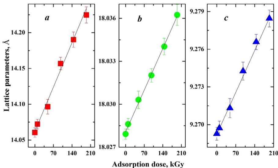
Fig. 3. Gamma irradiation dose dependences of lattice parameters of the orthorhombic phase of silicide hexboride at room temperature. Solid lines are interpolation of the experimental data by linear functions polynomials.
