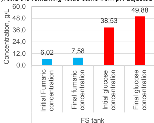
Figure 4: Changing of fumaric acid and glucose concentrations in the feed solution tank at 32 °C.
