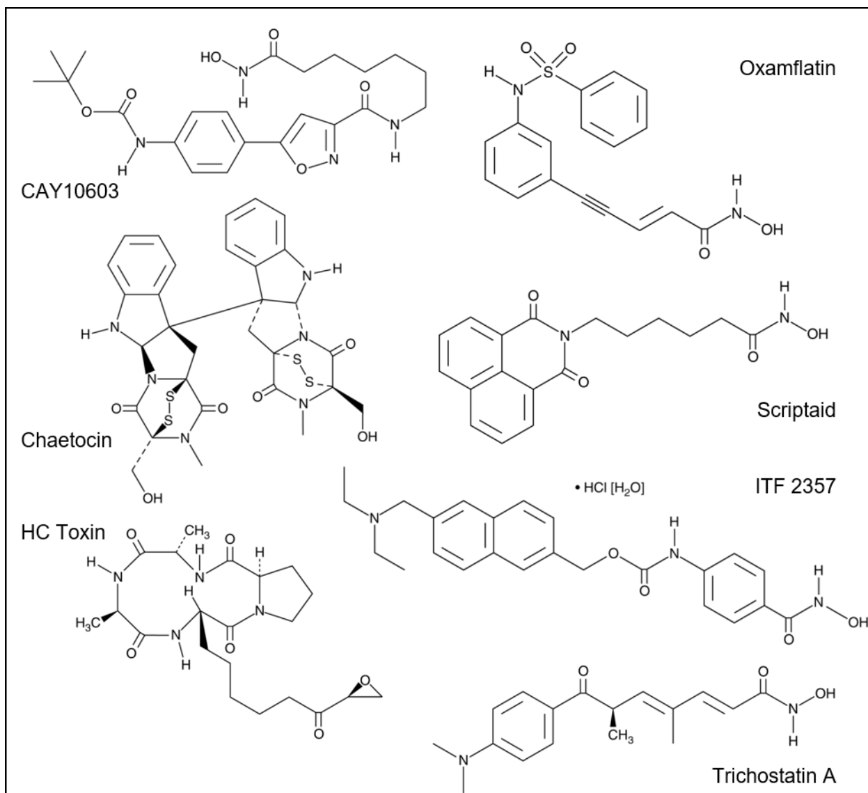
Figure A6: Chemical structures for unique structural compounds identified in the SALI plot.
