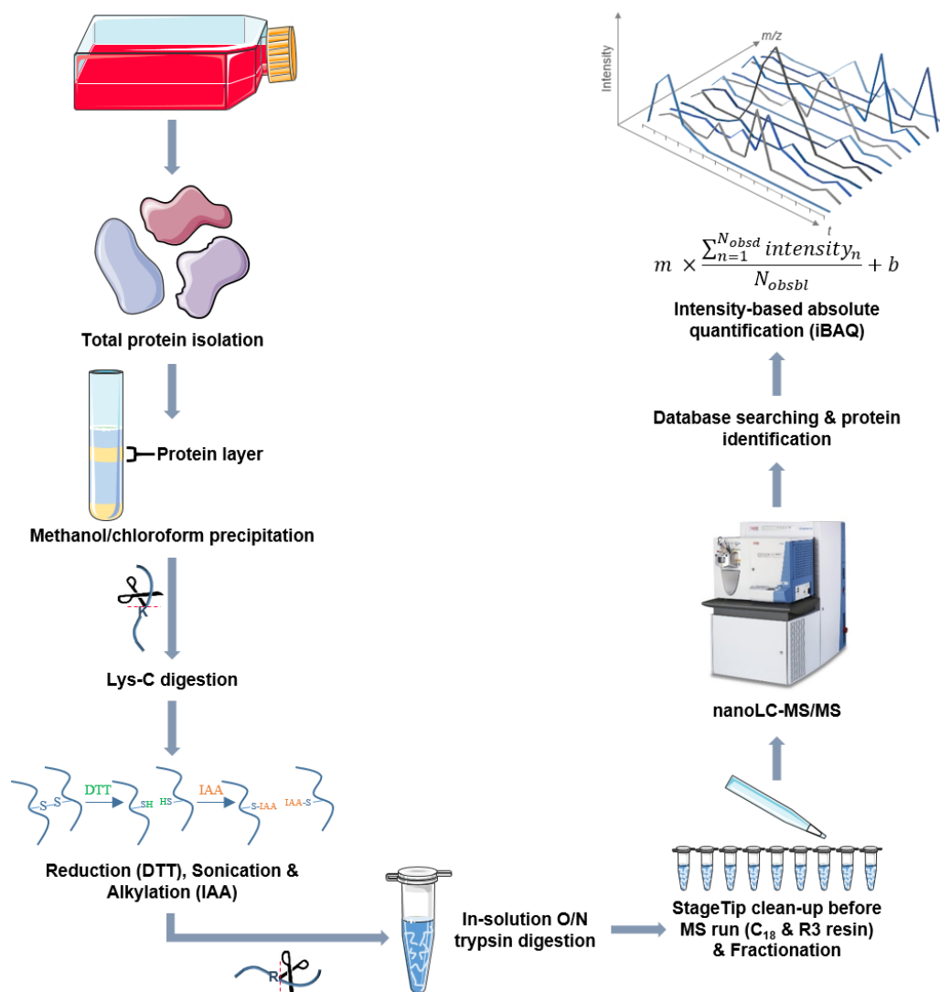
Figure 3.2: Quantitative proteomics approach. The proteins from each of the eight representative life cycle stages were isolated, precipitated, Lys-C digested, reduced (using DTT), sonicated, alkylated (using IAA), trypsin digested and finally cleaned up and fractionated for MS analysis. NanoLC-MS/MS was performed, followed by database searching and protein identification. Proteins were quantified using iBAQ. Images were adapted from Servier Medical Art (URL link to the license: https://creativecommons.org/licenses/by/3.0/ ) and changes were made in terms of colour and size.
