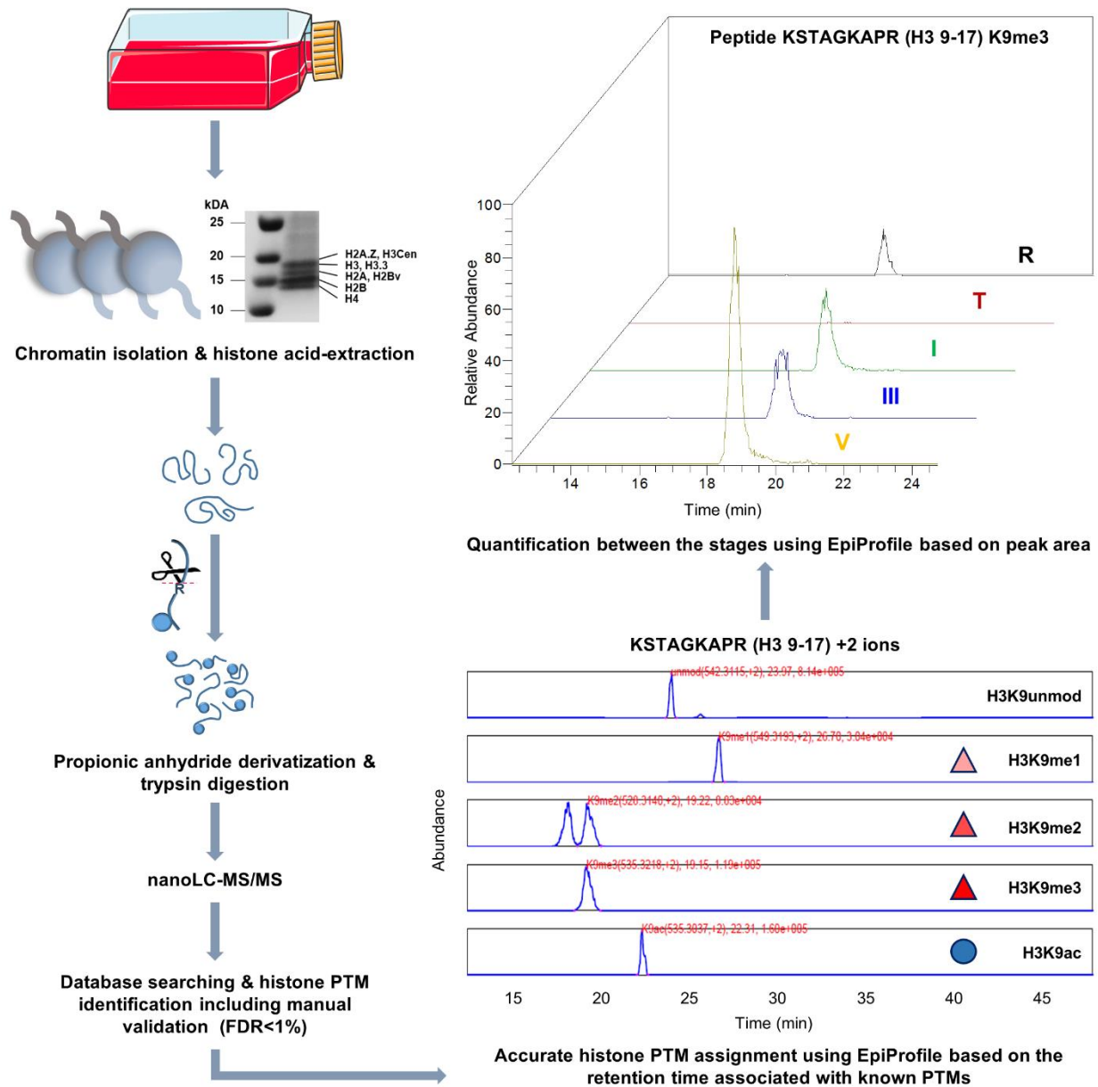
Figure 2.3: Chromatin proteomics approach for histone PTM quantification. The core and variant histones from each of the eight representative life cycle stages were acid-extracted, propionylated and trypsin digested. NanoLC-MS/MS was performed, followed by database searching and histone PTM identification including manual validation (FDR<1%). MS1 spectra of the P. falciparum histone H3 peptide KSTAGKAPR (aa 9-17), illustrating the discrimination between varying histone PTMs of H3K9 based on the retention time associated with known PTMs. After accurate PTM assignments, relative quantification using EpiProfile was performed, enabling accurate quantification of histone PTMs based on peak area and determination of co-existing PTMs on longer peptides. The abundance profiles during life cycle development were derived in this manner. The culture flask image was adapted from Servier Medical Art (URL link to the license: https://creativecommons.org/licenses/by/3.0/ ) and changes were made in terms of colour and size.
