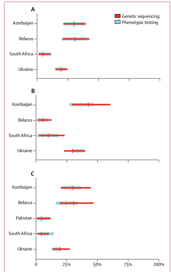
Figure 5: Prevalence of resistance to injectable kanamycin, amikacin, and capreomycin, estimated through genetic sequencing compared with phenotypic testing
