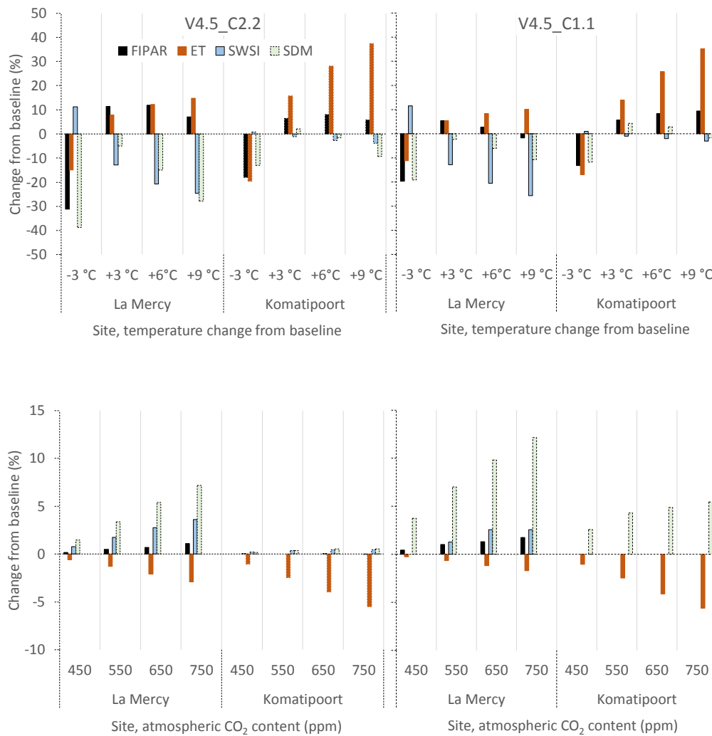
Figure 3. Change in long term mean (average for crops starting in April and October) seasonal interception of radiation (FiPAR), evapotranspiration (ET), photosynthesis/transpiration soil water satisfaction index (SWSI) and stalk dry mass at harvest (SDM) for different temperature regimes (-3, +3, +6, and +9 °C change from the baseline) and different atmospheric CO 2 levels (450, 550, 650 and 750 ppm) at La Mercy and Komatipoort, expressed as a percentage of that of the baseline regime, as simulated by the V4.5_C2.2 (left) and V4.5_C1.1 (right) models.
