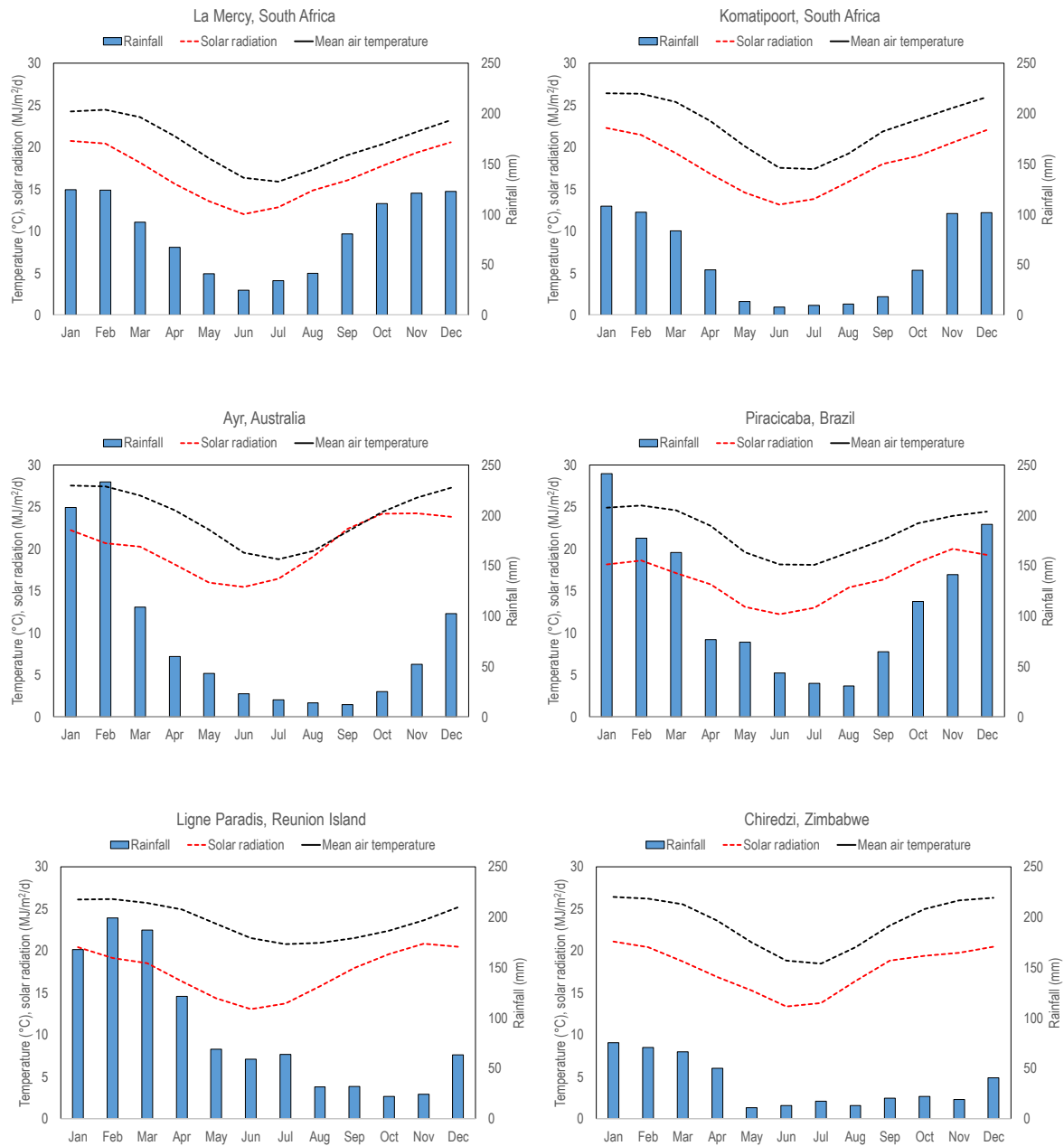
Figure 1. Long-term mean monthly rainfall, daily solar radiation and daily mean air temperature for the sites used for the climate change sensitivity analysis.
