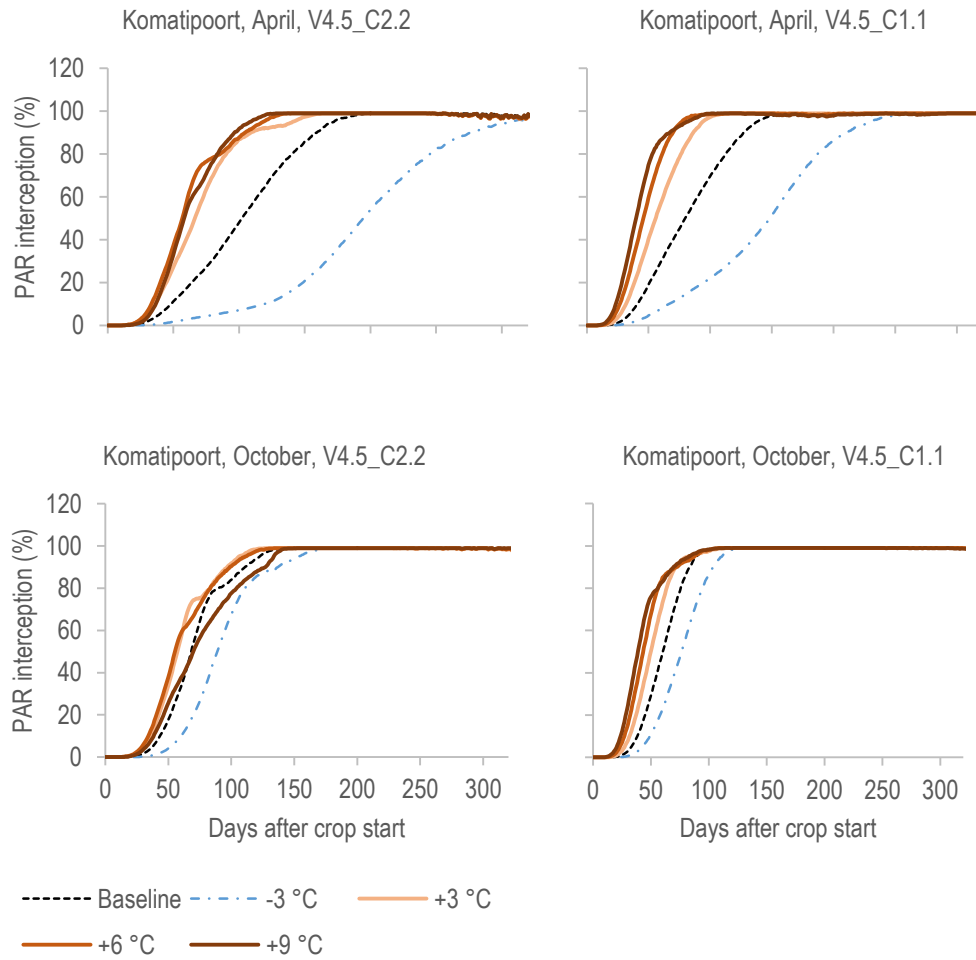
Figure 2. Long-term average fractional interception of PAR over the growing season for the different temperature regimes for crops started in April and October at Komatipoort, as simulated by V4.5_C2.2 (left) and V4.5_C1.1 (right) models.
