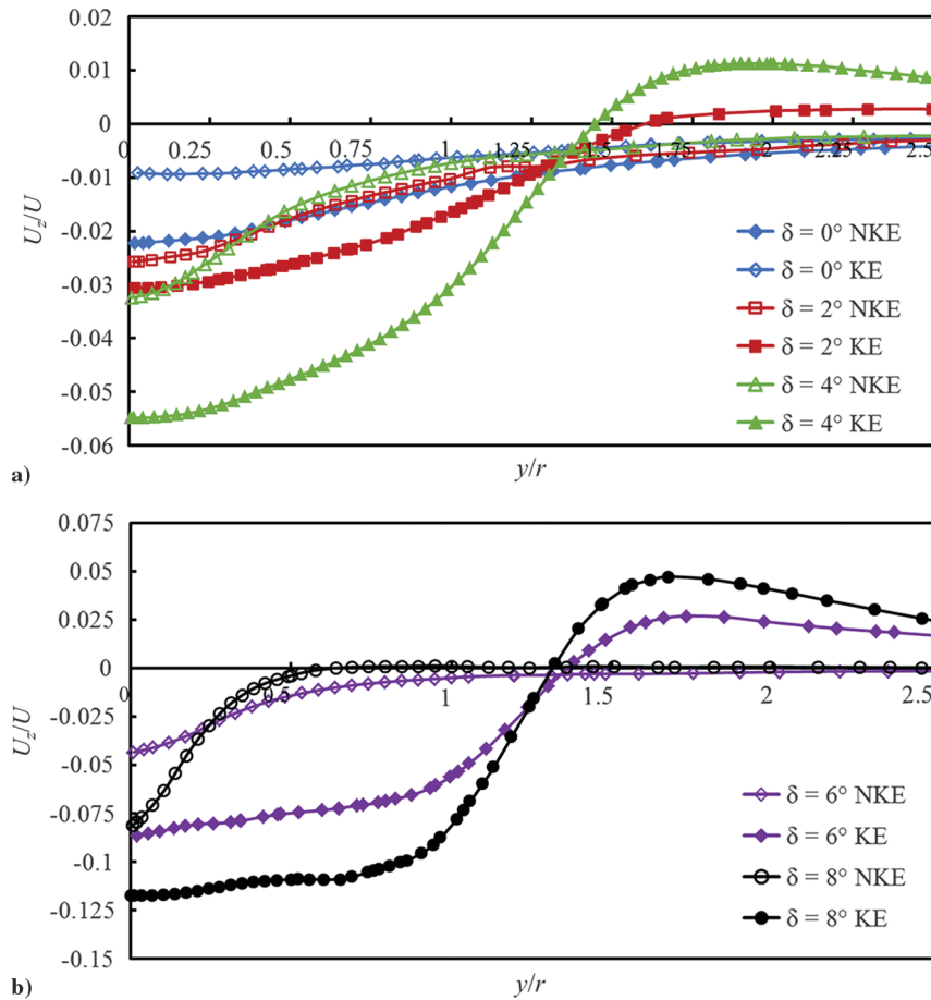
Fig. 10 U_z/U as a function of y/r , for the F-57 LDB: a) \delta = 0-4 deg, and b) \delta = 6 and 8 deg.
