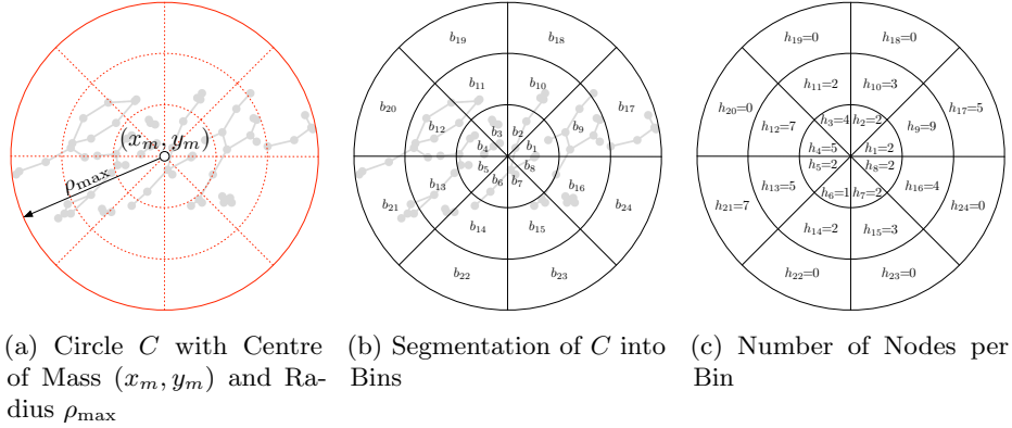
Fig. 1: Construction of the Polar Graph Dissimilarity.
