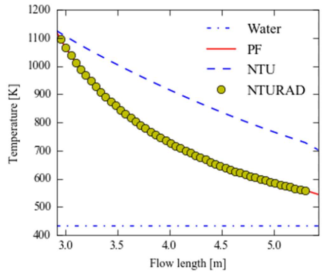
Figure 5 Temperature profile in the first tube pass for the PF, NTU and NTURAD models at low firing rate.
