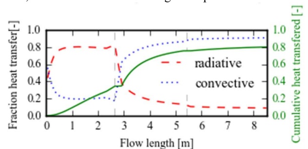
Figure 3 Fraction of heat transfer by radiation, convection and the cumulative heat transferred along the axial length at nominal load.
