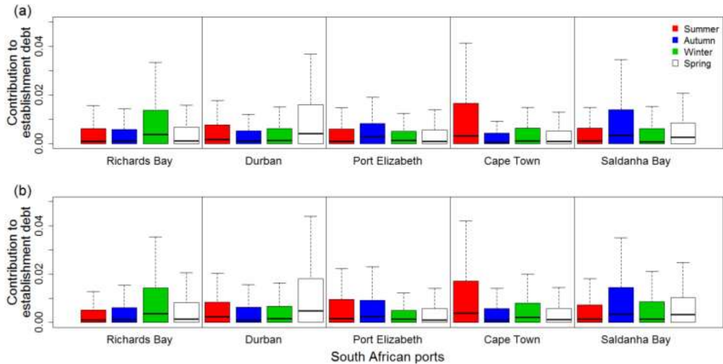
S7 Fig. The seasonal, relative contribution of shipping routes from foreign ports to the (a) marine and (b) terrestrial establishment debt of South African ports. Boxplots represent median and interquartile range. Seasons are based on those of the southern hemisphere.
