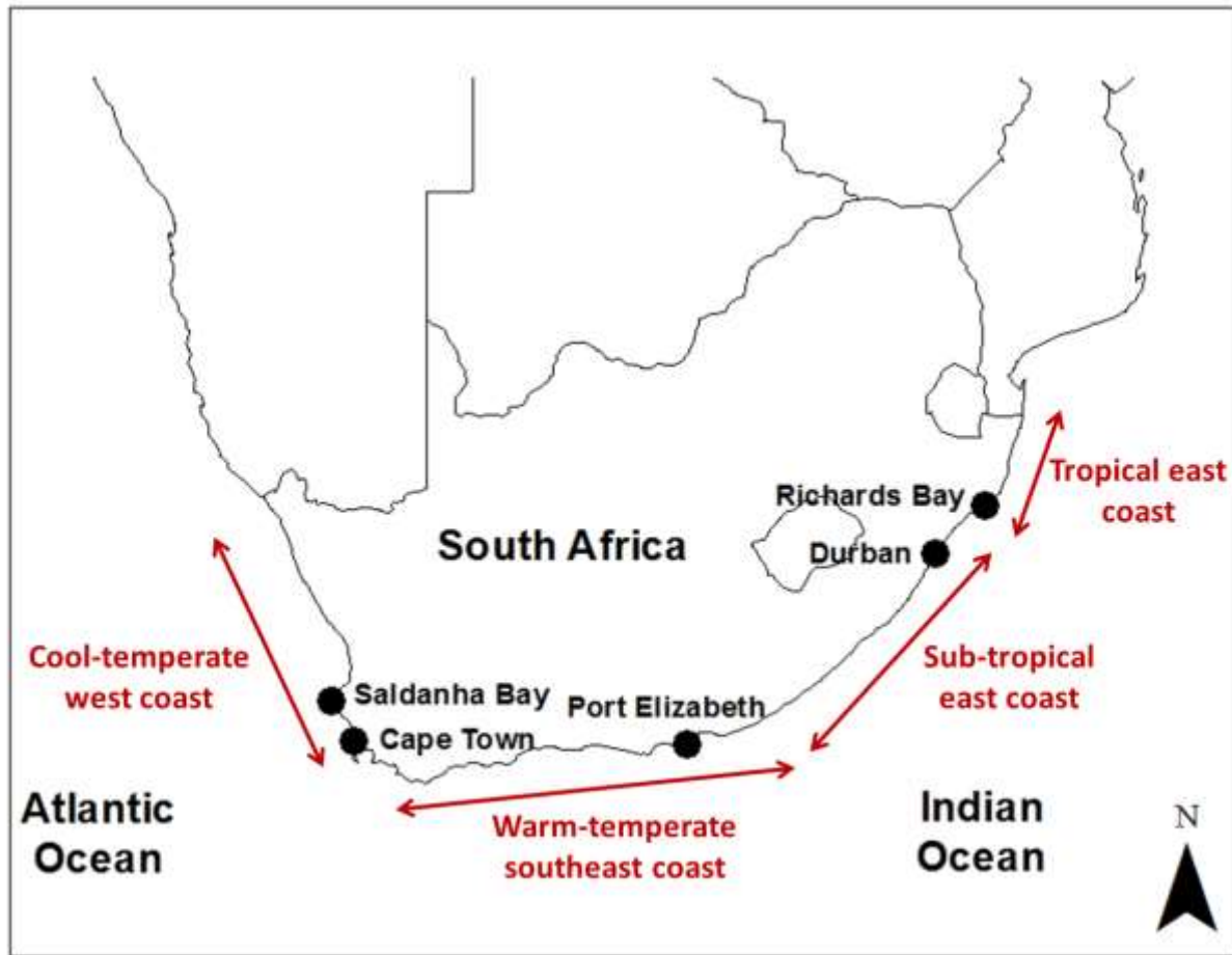
S5 Fig. The biogeographical regions (red) as classified by Mead et al. (2011) and the position of the five selected South African ports.
