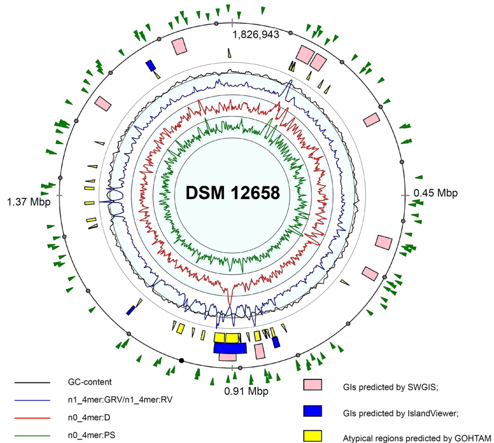
Figure 1. The genome and genomic islands (GI) of F. acidiphilum Y T . Localization of GIs on the chromosome of F. acidiphilum Y T , as predicted by SWGIS (pink boxes), IslandViewer (blue boxes) and GOHTAM (yellow boxes). Histograms in the inner cycles of the atlas depict variations of the following oligonucleotide usage parameters: GC-content (black curve); ratio of generalized to local relative variances calculated for tetranucleotide usage patterns normalized by the GC-content (blue curve, n1_4mer:GRV/n1_4mer:RV); distances between not-normalized local tetranucleotide usage pattern and the global one calculated for the complete chromosome (red curve, n0_4mer:D); asymmetry between not-normalized tetranucleotide usage patterns calculated for the direct and complement DNA strands (green curve, n0_4mer:PS). Use of these parameters for GI identification and their standard abbreviations were explained in more detail 68 . Green arrowheads (outer circle) indicate single-nucleotide substitutions in the genome of F. acidiphilum Y T after ~550 generations in the laboratory culture (s. Supplementary Table S2 for more details).
