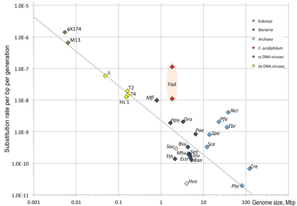
Figure 3. Single-nucleotide mutations accumulated during cultivation of F. acidiphilum Y T . Base-substitutional mutation rates per site per generation plotted vs genome sizes. The data on mutation rates of unicellular organisms and viruses and the regression plot ( \log_{10}u = -8.66 - 1.096\log_{10}G , where u and G are mutation numbers and genome size, respectively) are taken from 29 . Single-stranded DNA viruses: \phi X174, phage phi 174; M13, phage M13. Double-stranded DNA viruses: \phi , phage lambda; T2, phage T2; T4, bacteriophage T4; Hs 1, Herpes simplex virus. Bacteria: Bsu , Bacillus subtilis ; Ban , Bacillus anthracis ; Dra , Deinococcus radiodurans ; Hpy , Helicobacter pylori ; Mfl , Mesoplasma florum ; Mtu , Mycobacterium tuberculosis ; Pae , Pseudomonas aeruginosa ; Sen , Salmonella enterica ; Stu , Salmonella typhimurium ; Tth , Thermus thermophilus . Archaea: Fad , Ferroplasma acidiphilum ; Hvo , Haloferax volcanii ; Sac , Sulfolobus acidocaldarius . Eukarya: Cre , Chlamydomonas reinhardtii ; Ncr , Neurospora crassa ; Pfa , Plasmodium falciparum ; Sce , Saccharomyces cerevisiae ; Spo , Schizosaccharomyces pombe ; Tbr , Trypanosoma brucei ; Pte , Paramecium tetraurelia . Pink area reflects the distribution of mutation rates in Ferroplasma with the higher point value corresponding to all detected base substitutions in the strain cultured for ~550 generations as compared with the original genome, and lower value representing the most conservative mutation rate prediction (all mutations with frequency values <5% and SNPs in the original genome were excluded).
