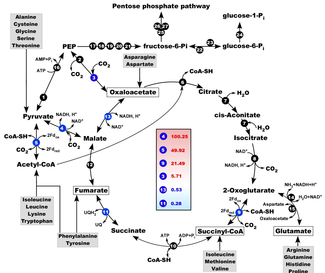
Figure 4. Proposed citric acid cycle and related enzyme reactions in F. acidiphilum Y T . The enzymes are as follows: 1, pyruvate kinase (FAD_1603); 2, PEP carboxykinase (FAD_1050); 3, PEP carboxylase (FAD_1044); 4, NAD-binding malic enzyme/malate dehydrogenase (FAD_0703); 5, pyruvate: ferredoxin oxidoreductase (FAD_0567–0568); 6, citrate synthase (FAD_1100); 7, aconitate hydratase (FAD_0701); 8, isocitrate dehydrogenase (FAD_1632); 9, 2-oxoglutarate:ferredoxin oxidoreductase (FAD_0712–0713); 10, succinyl-CoA synthetase (FAD_0709–710); 11, succinate dehydrogenase (FAD_0714–0717); 12, fumarate hydratase (FAD_1630); 13, malate dehydrogenase (FAD_0718); 14, glutamate dehydrogenase (FAD_0434); 15, aspartate aminotransferase (FAD_1098); 16, phosphoenolpyruvate synthase (FAD_1233); 17, phosphoglycerate mutase (FAD_0440, FAD_1169, FAD_1350); 18, 2-phosphoglycerate kinase (FAD_1810); 19, glyceraldehyde-3-phosphate dehydrogenase (FAD_0549); 20, triosephosphate isomerase (FAD_0107); 21, fructose-2,6-bisphosphatase (FAD_0332); 22, 6-phosphofructokinase (FAD_0353); 23, bifunctional phosphoglucose/phosphomannose isomerase (FAD_0562); 24, phosphoglucomutase/phosphomannomutase (FAD_0602); 25, transketolase (FAD_1477–1476); 26, transaldolase (FAD_1201; FAD_1475); 27, ribulose-phosphate 3-epimerase (FAD_0295). Abbreviations used: Fd, electron carrier ferredoxin; NAD, nicotinamide adenine dinucleotide; CoA, Coenzyme-A; PEP, phosphoenolpyruvate; UQ, ubiquinone. Enzymes labeled in blue are potentially involved in anaplerotic assimilation of CO 2 . Their relative expression levels, analysed by RT-qPCR and indicated by the numbers in the central box, were obtained by normalization of the total RNA added and using transcripts of DNA gyrase subunit B ( gyrB ) as the internal reference (value 1.0). Normalization using gyrB was additionally validated vs transcripts of gene for ribosomal L2 protein. Average normalisation data derived from triplicates with standard deviation below 5%.
