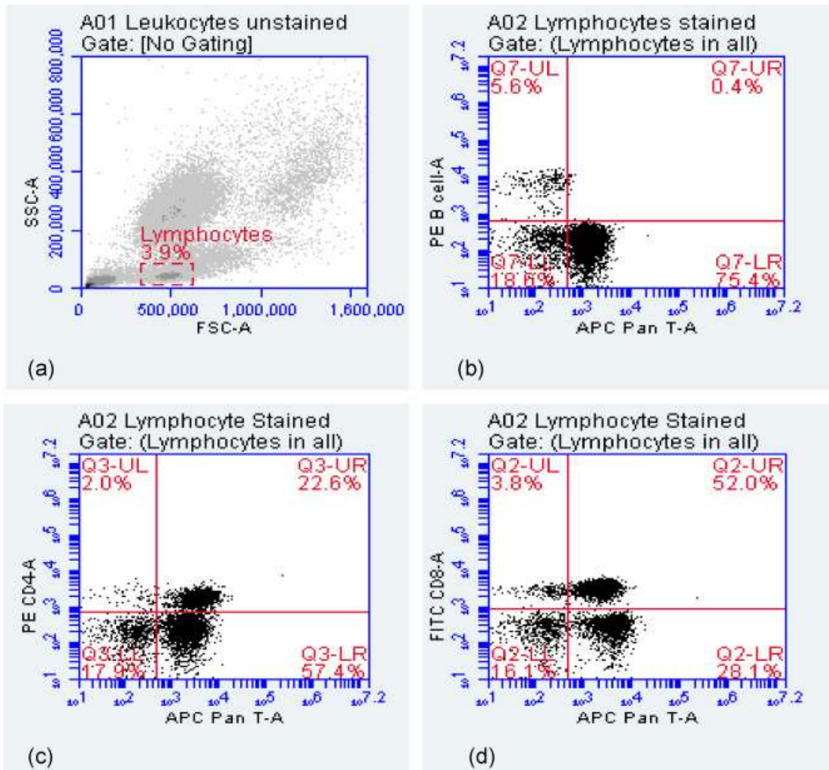
Fig. 1 Flow cytometric analysis of peripheral lymphocyte phenotypes. (a) The lymphocyte population was identified and gated based on forward-angle and side-angle light scatter characteristics of unstained cells. (b – d) Subsequently the lymphocytes were gated on their CD3 (in APC) (b), B cell marker (in PE) (b), CD4 (in PE) (c), or CD8 (in FITC) (d) expression. Values in the quadrant indicate the percentage of cells.
