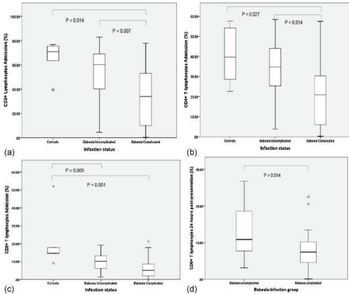
Fig. 2 Box plots of the CD3 + lymphocyte (a), CD4 + T lymphocyte (b), and CD8 + T lymphocyte (c) percentages in the healthy control group of dogs and the Babesia -infected dogs with uncomplicated and complicated disease at admission, and the 24 hours post-presentation CD8 + lymphocyte percentages in the Babesia -infected dogs with uncomplicated and complicated disease (d). The box represents the interquartile range (IQR), the line represents the median, the upper and lower whiskers represent values within 1.5xIQR of the 75 th and 25 th percentiles respectively; outliers are plotted as open circles and asterisks represent extreme outlier values that are 3 times removed from the IQR.
