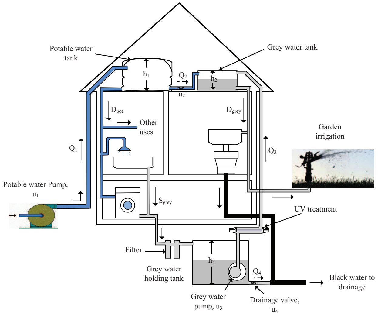
Figure 1: Schematic of water pumping and grey water recycling system
