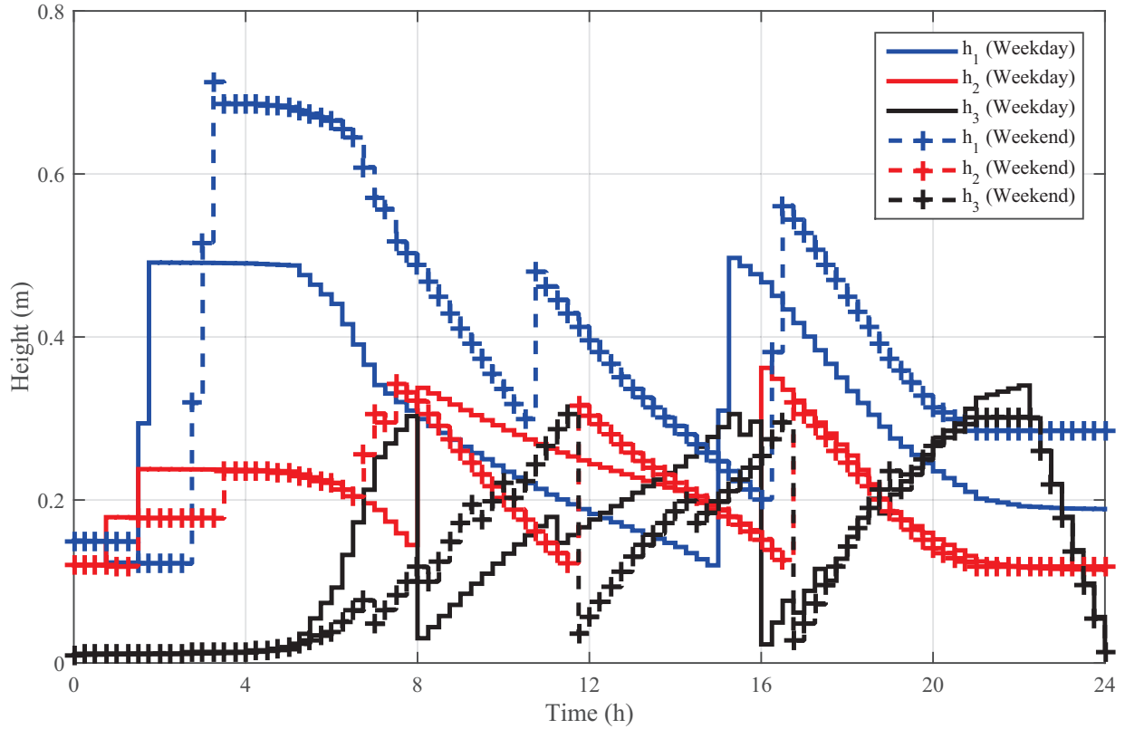
Figure 8: Water height variation using MPC controller.
