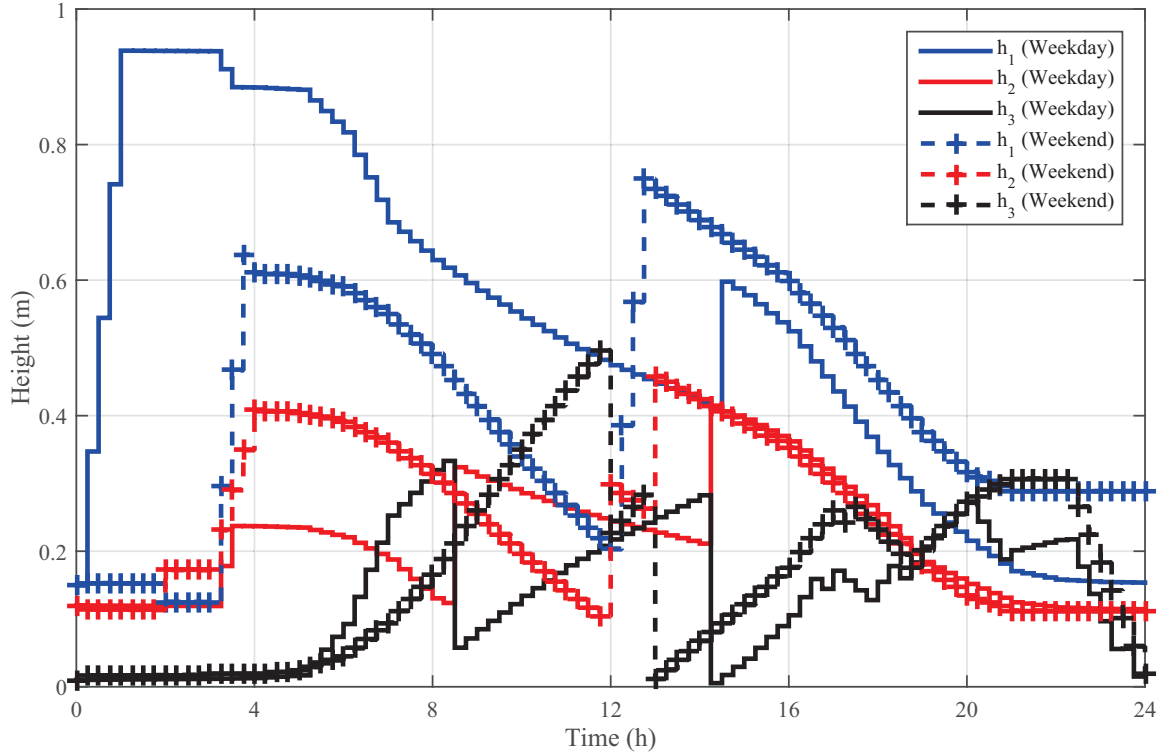
Figure 5: Water height variation in respective tanks with open loop controller.
