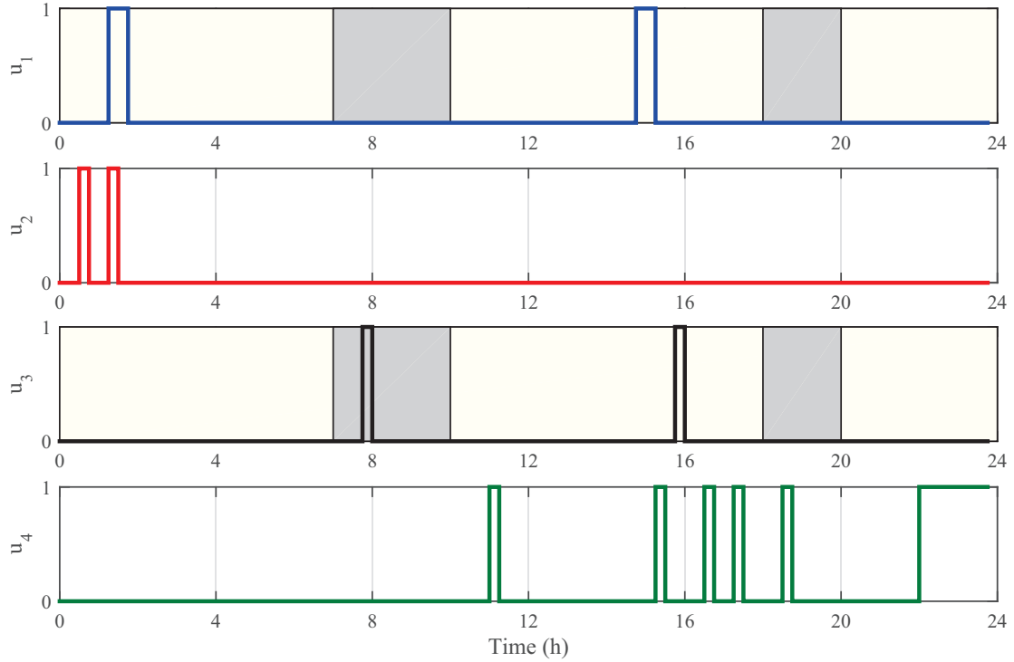
Figure 6: Week day closed-loop optimal switching.
