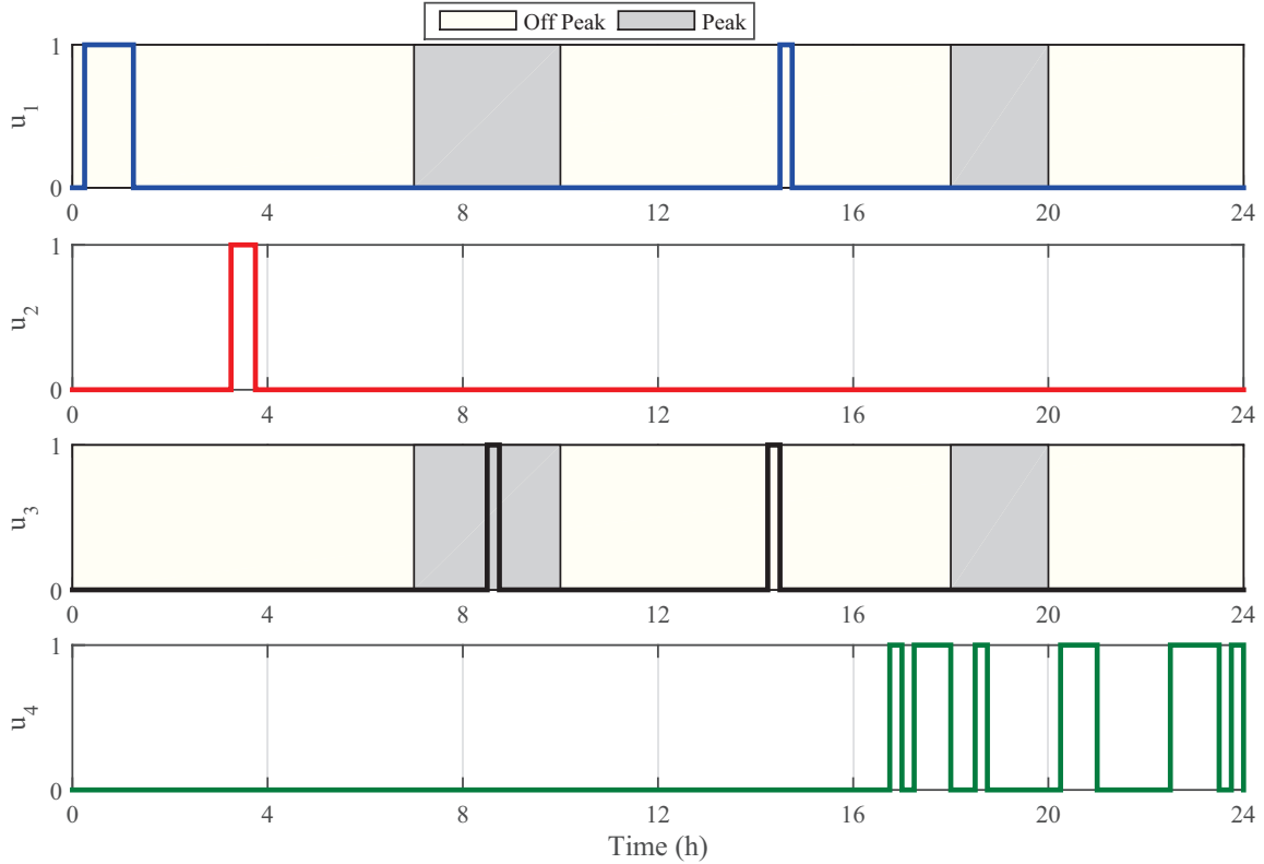
Figure 3: Open loop optimal switching for a weekday.
