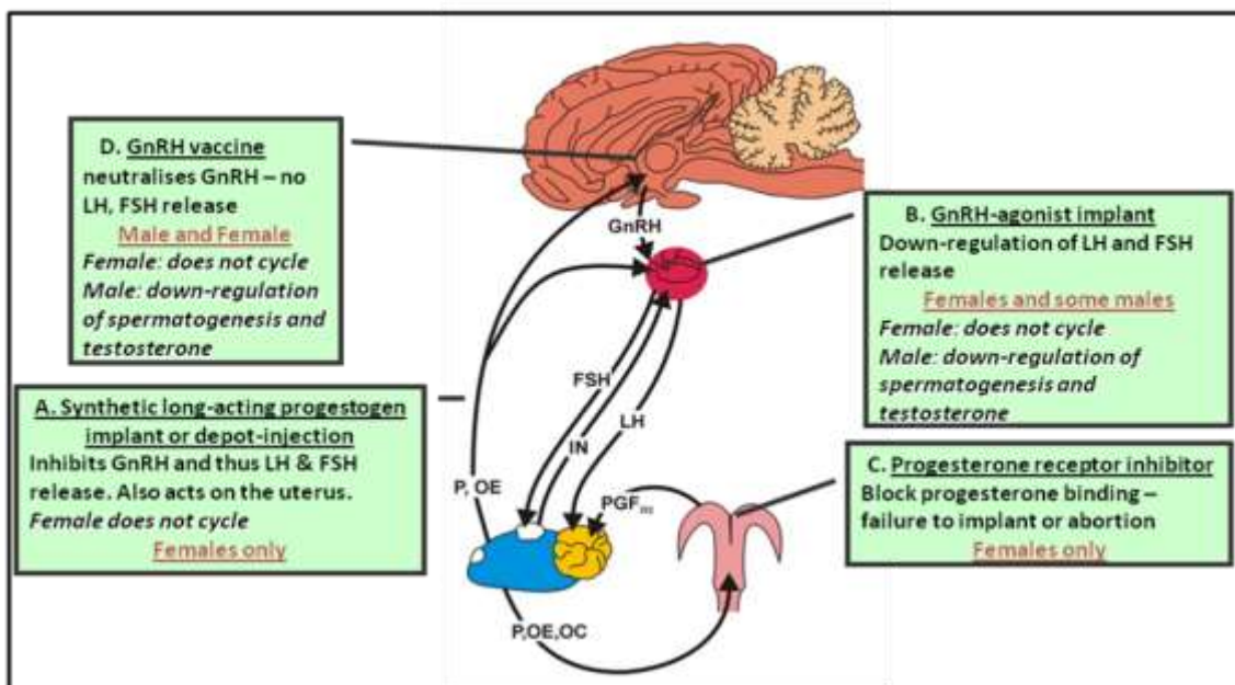
Fig. 1. Endocrine control of female reproduction and mechanism of action of progestins (A), GnRH-agonists (B), progesterone receptor inhibitors (C) and GnRH vaccines (D) (modified from Bertschinger et al. 2008b).
