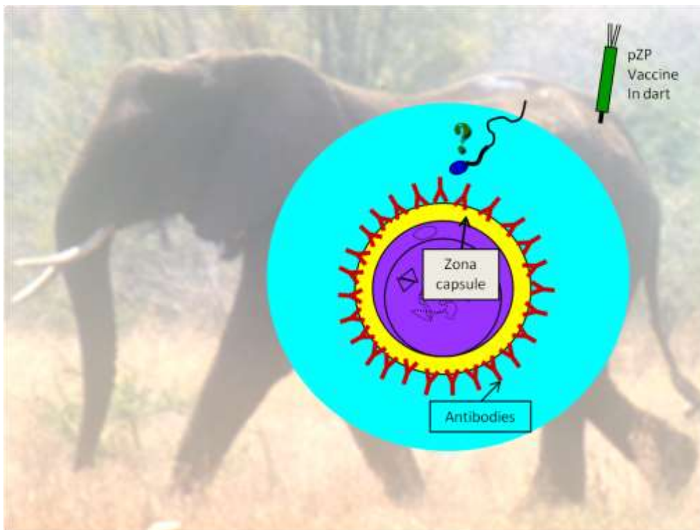
Fig. 4. Mechanism of action of the pZP vaccine
