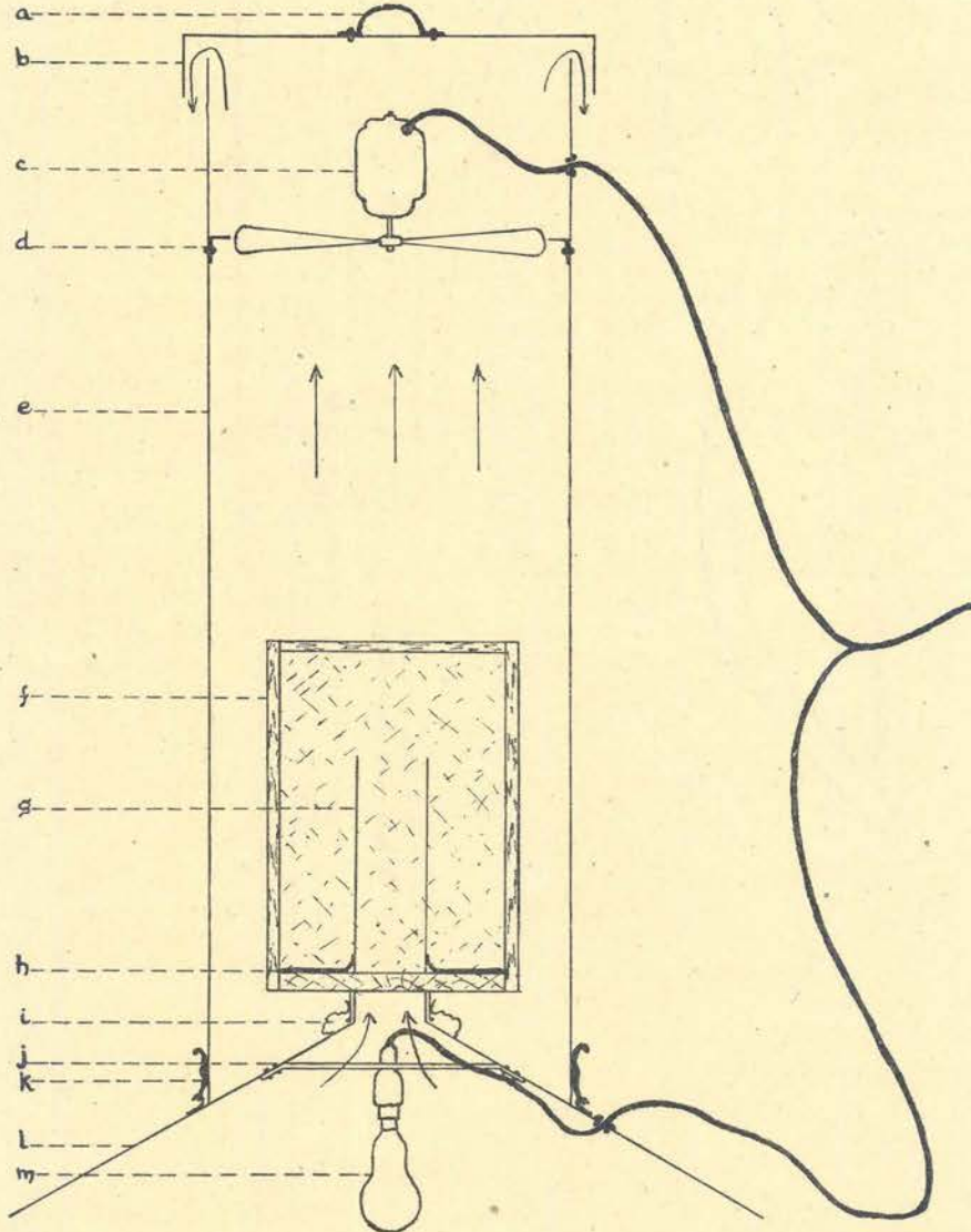
Fig. 1.—Light trap. (a) Metal loop for suspending trap. (b) Dustbin type cover. (c) Electric fan with 7 in. blades. (d) Metal flange to allow \frac{1}{8} in. clearance for fan blades. (e) Cylindrical sheet metal body of trap. 8 in. diameter. (f) Catching cage. (g) Sheet metal inlet pipe or tube. (h) Felt or thick woollen cloth glued around opening of catching cage to act as seal between this opening and inlet tube. (i) Muslin sleeve. (j) Metal bracket to support lamp. (k) Spring clip attaching conical hood to body of trap. (l) Conical sheet metal hood 17 in. wide below. (m) 75 watt electric lamp. Arrows indicate direction of air flow.
