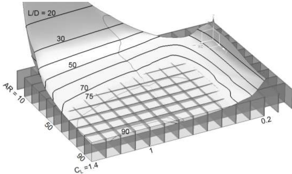
Figure 4 The surface of D/L as a function of AR and C_L shows, by means of the L/D contours, how C_L and AR should increase to get to the best performance (with the lowest region offering the best L/D ). The fissure in the otherwise smooth surface separates two different flap settings.
