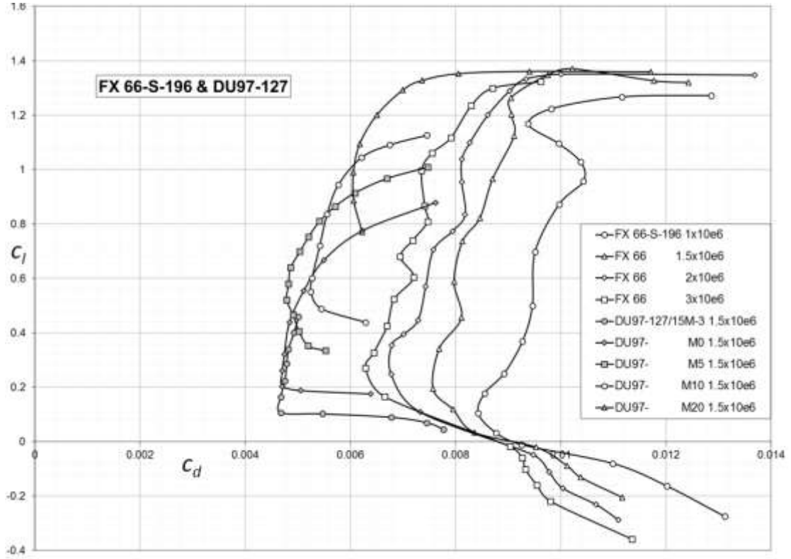
Figure 3 Experimental data of the Wortmann FX 66 aerofoil [22] at different Reynolds numbers and the Delft DU97 aerofoil [19] at different flap settings. For each polar curve, only the laminar ‘drag bucket’ is shown.
