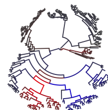
Supplementary Figure 5. Leading principal components correspond to major lineages in bacterial genealogies. For each species, branches of the maximum likelihood phylogeny are coloured by their correlation with each of PCs 1-5. Positive vs. negative correlations are shown in red vs. blue, brighter colours indicating stronger correlation. A square root transform was applied to branch lengths to visualize fine-scale structure.
