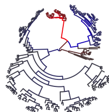
Supplementary Figure 5. Leading principal components correspond to major lineages in bacterial genealogies. For each species, branches of the maximum likelihood phylogeny are coloured by their correlation with each of PCs 1-5. Positive vs. negative correlations are shown in red vs. blue, brighter colours indicating stronger correlation. A square root transform was applied to branch lengths to visualize fine-scale structure.
