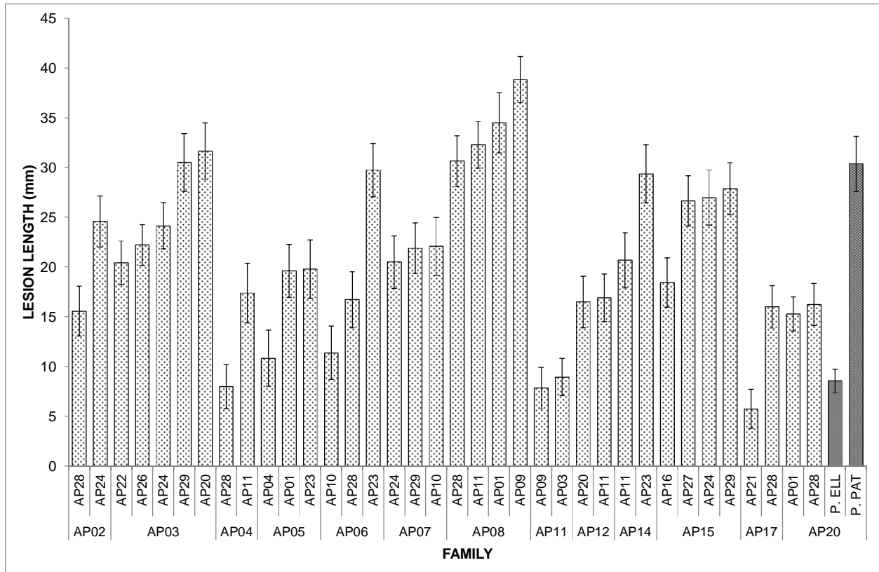
Figure 3. The variation in tolerance among P. patula full-sib families, which share a common female parent, relative to the P. elliotii and P. patula seedling control.
