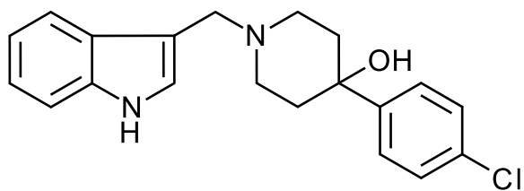
L,741,626
