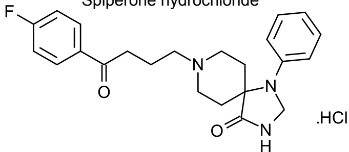
Spiperone hydrochloride
