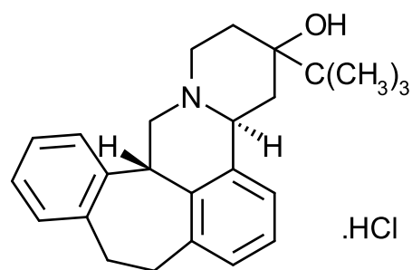
(+)-butaclamol hydrochloride
