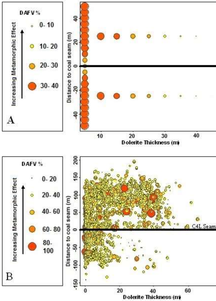
Figure 5: Dry ash free volatile percentage % (DAFV%) values in relation to the thickness of dolerite and the interval between the dolerite and the coal seam for all dolerites in the study area.
