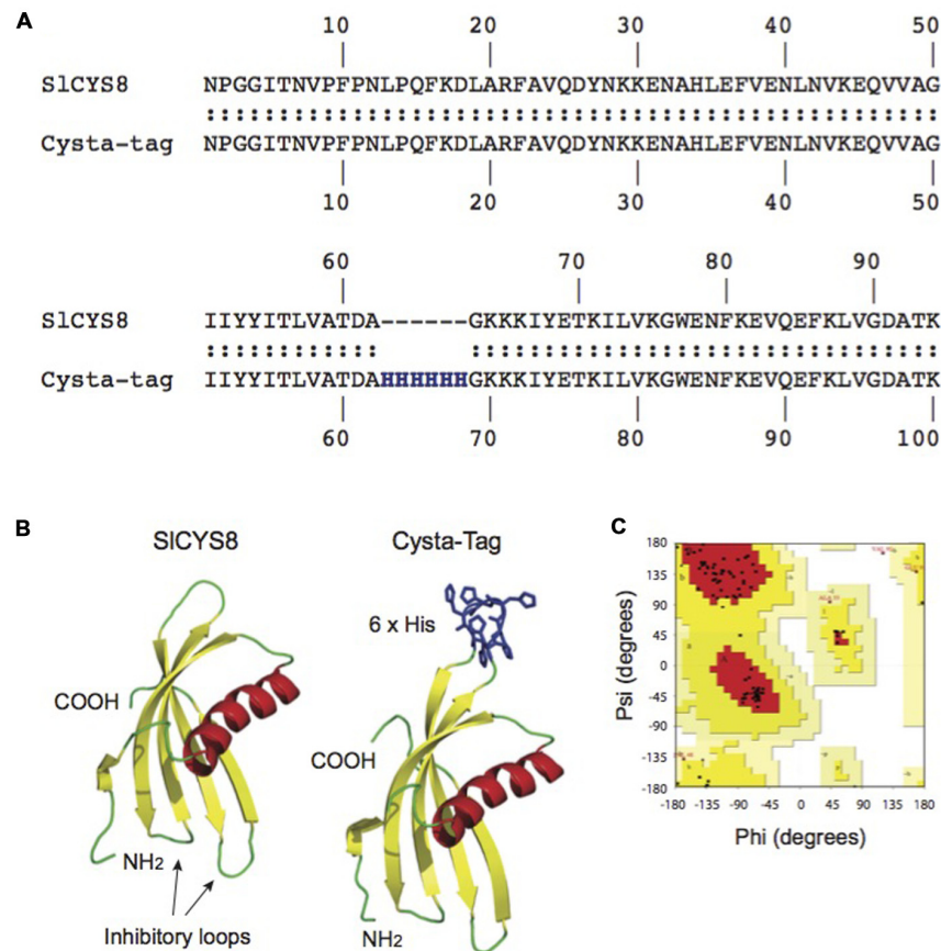
FIGURE 1 | In silico modeling of the Cysta-tag. Computationally modeling putative His-motif variants of S1CYS8 based on the NMR solution structure of oryzacystatin-I (PDB 1EQK) identified surface loop residues Ala-62 and Gly-63 as a possible target site for (His) 6 motif insertion with minimal impact on the template structure (A) . Graphical representation of the in silico models shows location of the poly-His motif at this position, away from the N-terminus and inhibitory loops involved in protease inhibition (B) . A Ramachandran plot produced with PROCHECK for the 'Ala-62-(His) 6 -Gly-63' Cysta-tag model (C) shows more than 90% of the amino acid residues (black dots) to fall within the 'most favored' (red) and 'additional allowed regions' (yellow) areas of the graph, as expected for good quality structural models (Morris et al., 1992).
