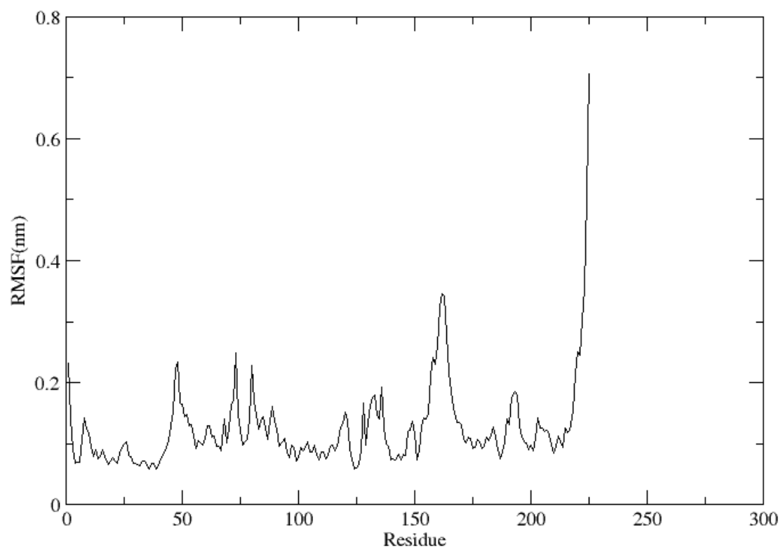
Figure S8 – RMS fluctuations of all C \alpha residues for the Rv1712 over the 30000ps simulation.
