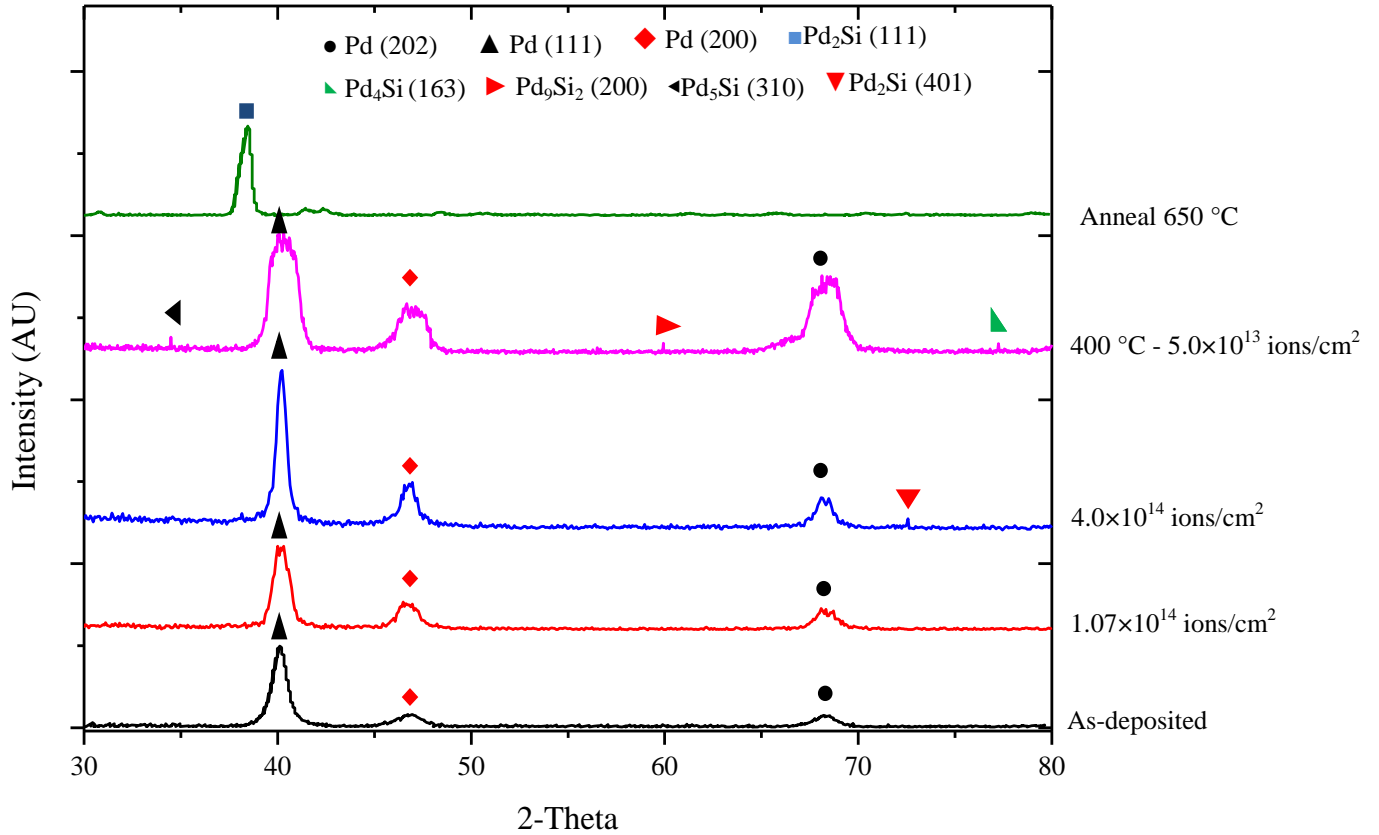
Figure 3: GIXRD pattern of as-deposited Pd/SiC, after RT irradiation at fluences of 1.07 \times 10^{14} and 4 \times 10^{14} , 5 \times 10^{13} ions/cm 2 at 400 °C and after in situ annealing at temperature of 650 °C.
