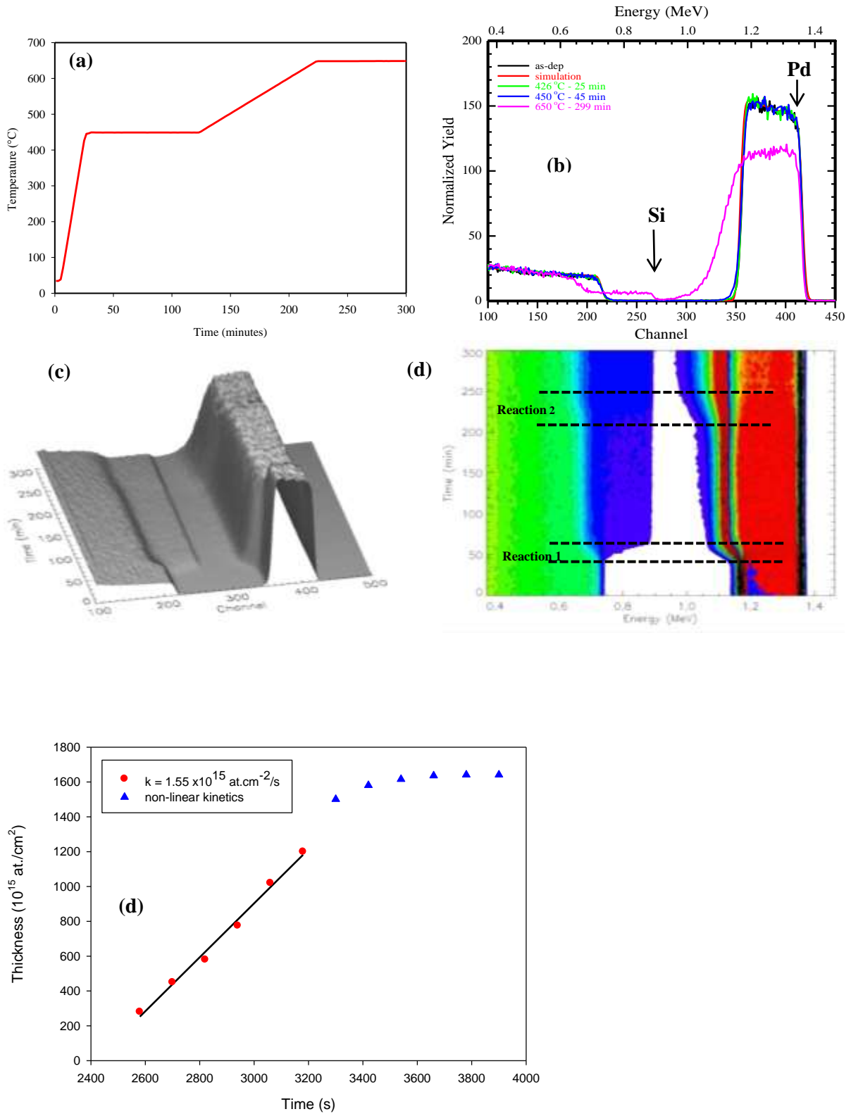
Figure 1: (a) Different temperature ramp anneal used for in situ annealing (b) overlay of RBS spectra and simulation of as-deposited and annealed samples (c) three dimensional plot of RBS spectra (d) contour lines of RBS spectra obtained during in situ RBS analysis (e) plot of reaction zone thickness versus time during Reaction 1 at 450 °C.
