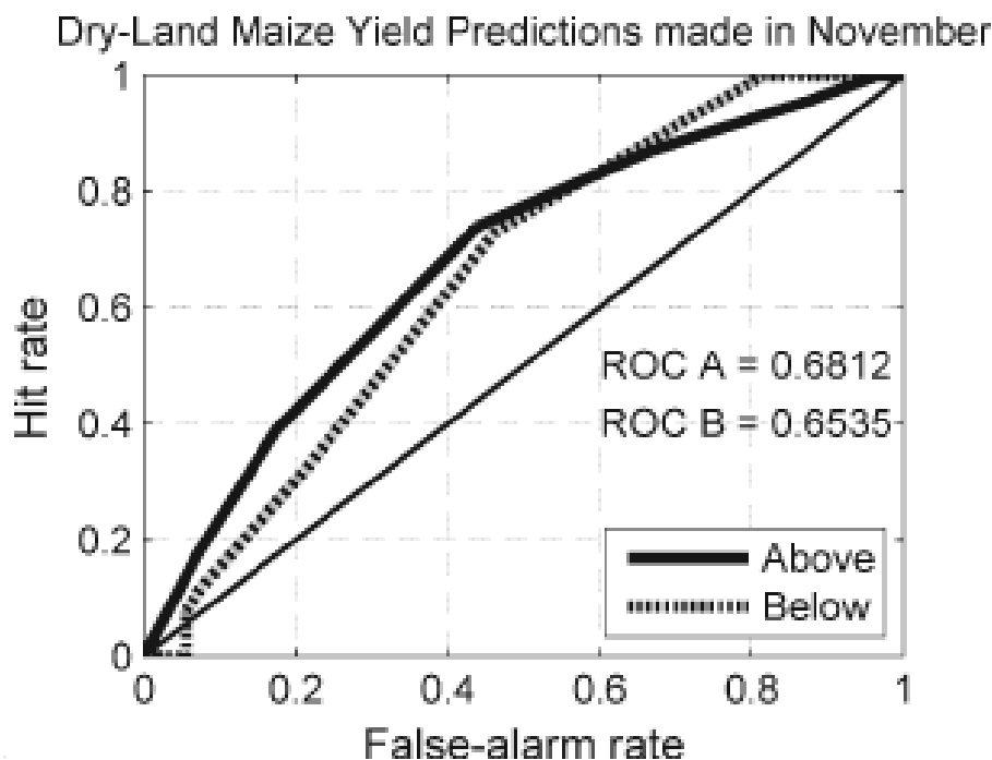
Figure 5. Relative operating characteristic curves for above- (>67 th percentile; thick solid curve) and below- (<33 rd percentile; thick dashed curve) normal maize yield hindcasts produced by downscaling SINTEX-F DJF 850 hPa geopotential height fields to agricultural districts over north-eastern South Africa, and associated areas beneath each curve
