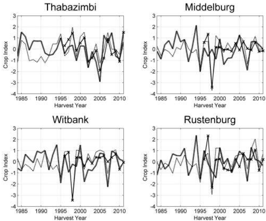
Figure 3. Observed (detrended, thick dashed lines) maize yield indices for four agricultural districts over north-eastern South Africa, and associated cross-validated (thin dashed line) and retro-active (solid lines and crosses) downscaled hindcasts. The years indicated represent the year of harvesting
