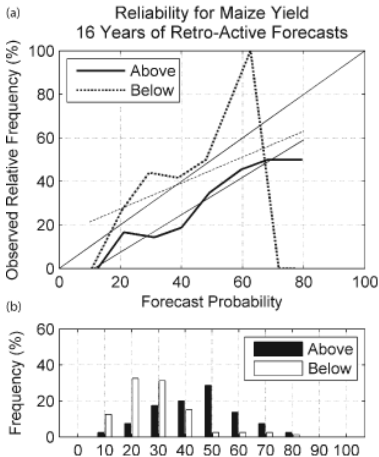
Figure 6. Reliability diagram (top) and frequency histogram (bottom) for above- (>67 th percentile) and below- (<33 rd percentile) normal maize yield hindcasts produced by downscaling SINTEX-F DJF 850 hPa geopotential height fields to agricultural districts over north-eastern South Africa. The thick solid (dashed) curve and the black (white) bars represent the high- (low-) yield category. The thin solid (dashed) line is the weighted least squares regression line of the high- (low-) yield reliability curve
