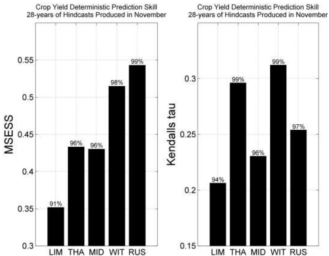
Figure 4. Mean squared error skill scores obtained by using persistence as reference hindcasts (left-hand panel) and Kendall's tau values (right-hand panel). The statistical significance for each score is shown on top of each bar. The significance values are obtained through a Monte Carlo rerandomization process
