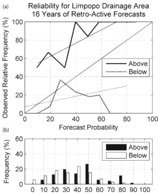
Figure 8. Reliability diagram (top) and frequency histogram (bottom) for above- (>67 th percentile) and below- (<33 rd percentile) normal streamflows of the Limpopo drainage area hindcasts produced by downscaling SINTEX-F DJF 850 hPa geopotential height fields to six flow-gauges. The thick solid (dashed) curve and the black (white) bars represent the high- (low-) yield category. The thin solid (dashed) line is the weighted least squares regression line of the high- (low-) yield reliability curve
