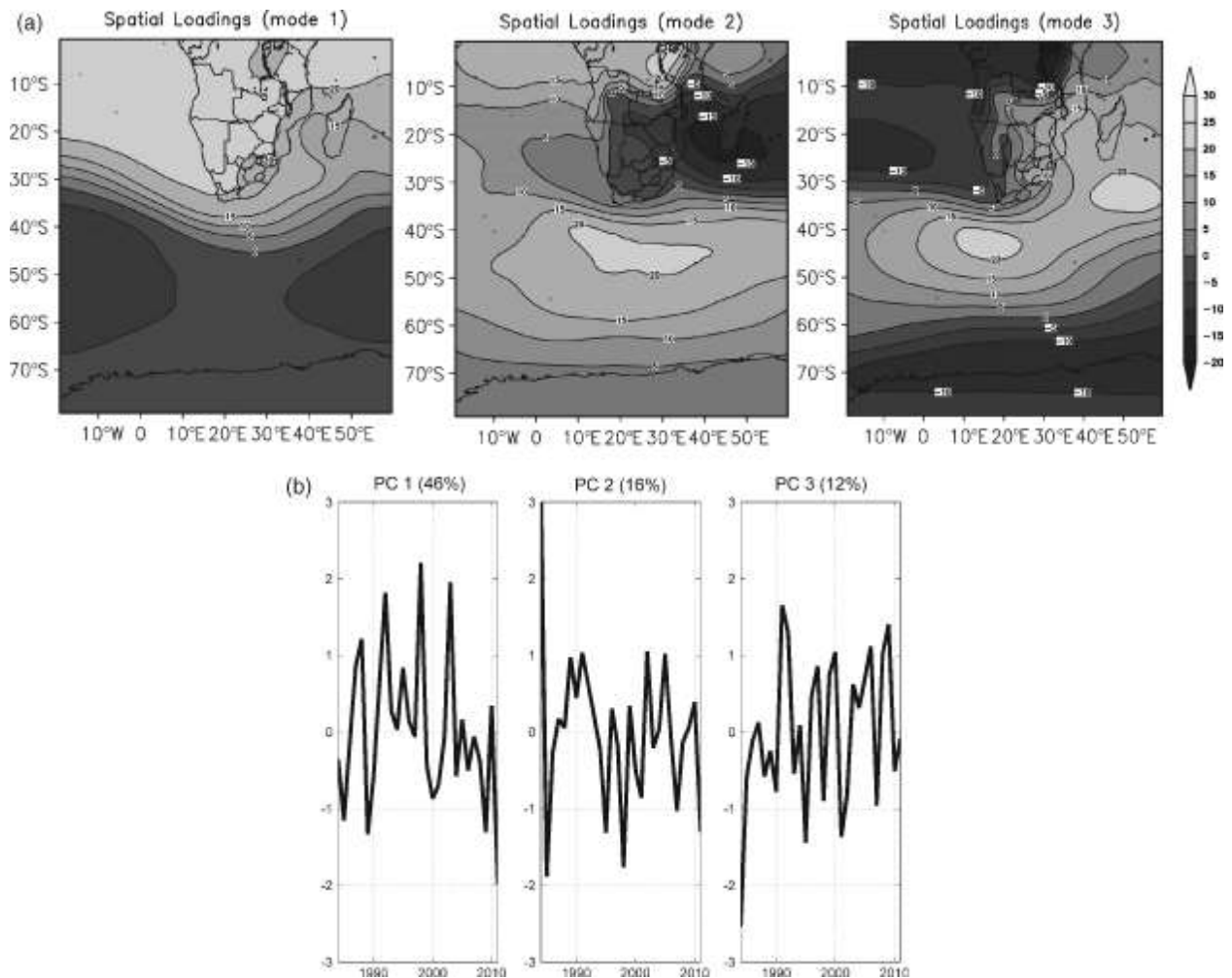
Figure 2. (a) The first three dominant PCA spatial loadings of the SINTEX-F's DJF 850 hPa geopotential height field for the 28-year period of 1983/84 to 2010/11. (b) The temporal scores associated with the loadings (a). The explained variance of each mode is also presented
