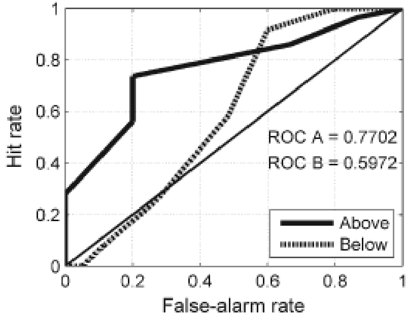
Figure 7. Relative operating characteristic curves for above- (>67 th percentile; thick solid curve) and below- (<33 rd percentile; thick dashed curve) normal streamflows of the Limpopo drainage area hindcasts produced by downscaling SINTEX-F DJF 850 hPa geopotential height fields to six flow-gauges, and associated areas beneath each curve
