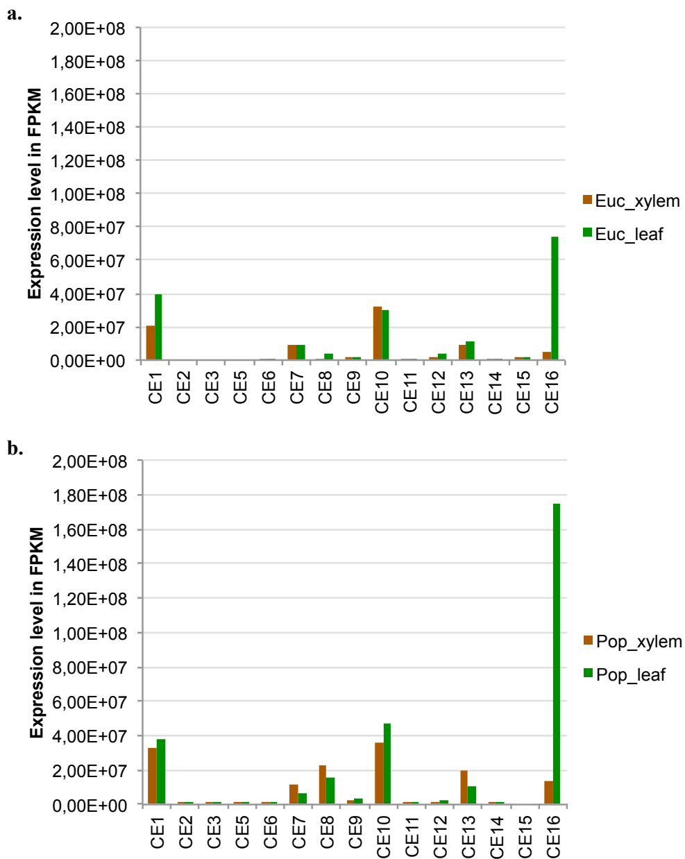
Figure S10 Comparative expression patterns of CE domain families in E. grandis and P. trichocarpa .
