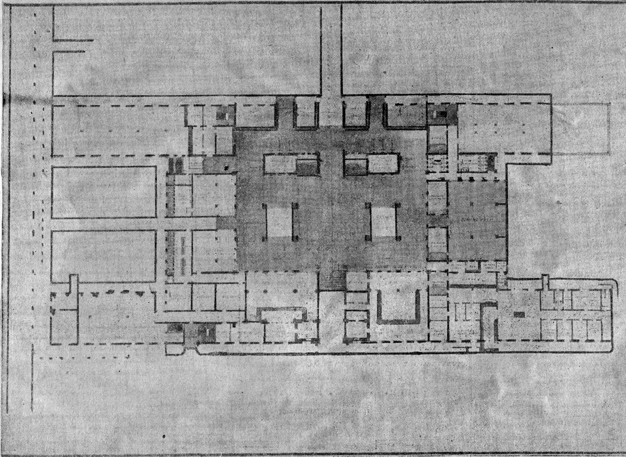
Plan of lower ground floor or concourse level. The waiting rooms are situated in the centre of the square. On the left is the subway to the Wanderers.
