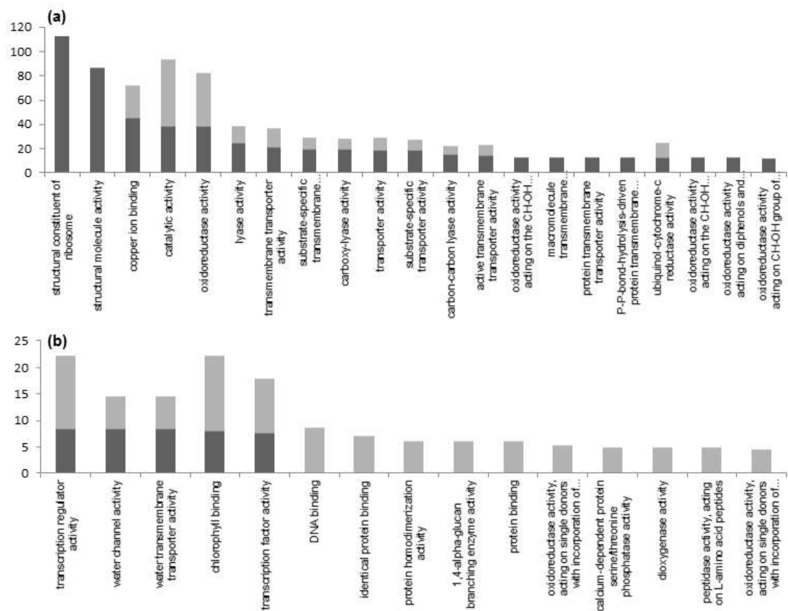
Additional file 3: Figure S1.. Molecular function GO terms that are over-represented in TAG5 and ZG14. a – GO terms within the up-regulated dataset. b – GO terms within the down-regulated dataset (all terms for this dataset are shown). The y-axis represents the -\log_2(q\text{-value}) and the x-axis represents the GO terms within the datasets. Light and dark grey bars are ZG14 and TAG5 respectively.
