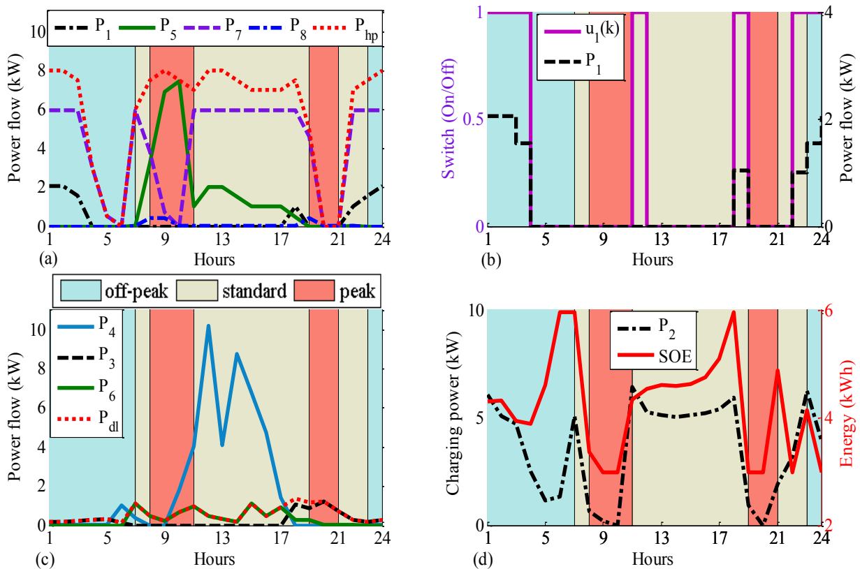
Figure 4: (a) OC of power to the HPWH; (b) OC switching to the HPWH; (c) Domestic load and solar sales ;(d) Battery SOE
