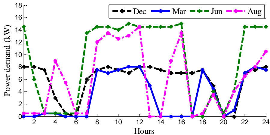
Figure 2: HPWH hourly demand (kW)
