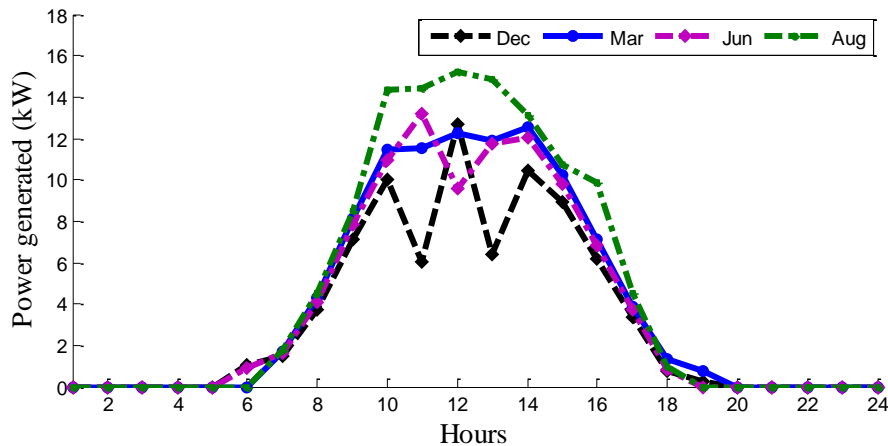
Figure 3: PV power output (kW)
