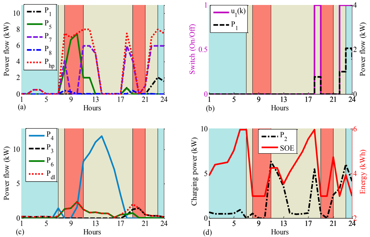
Figure 5: (a) OC of power to the HPWH; (b) OC switching to the HPWH; (c) Domestic load and solar sales ;(d) Battery SOE
