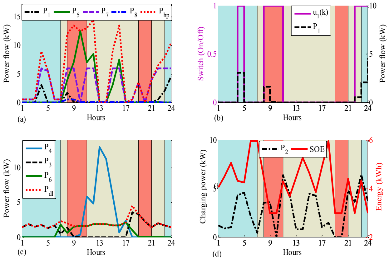
Figure 7: (a) OC of power to the HPWH; (b) OC switching to the HPWH; (c) Domestic load and solar sales ;(d) Battery SOE
