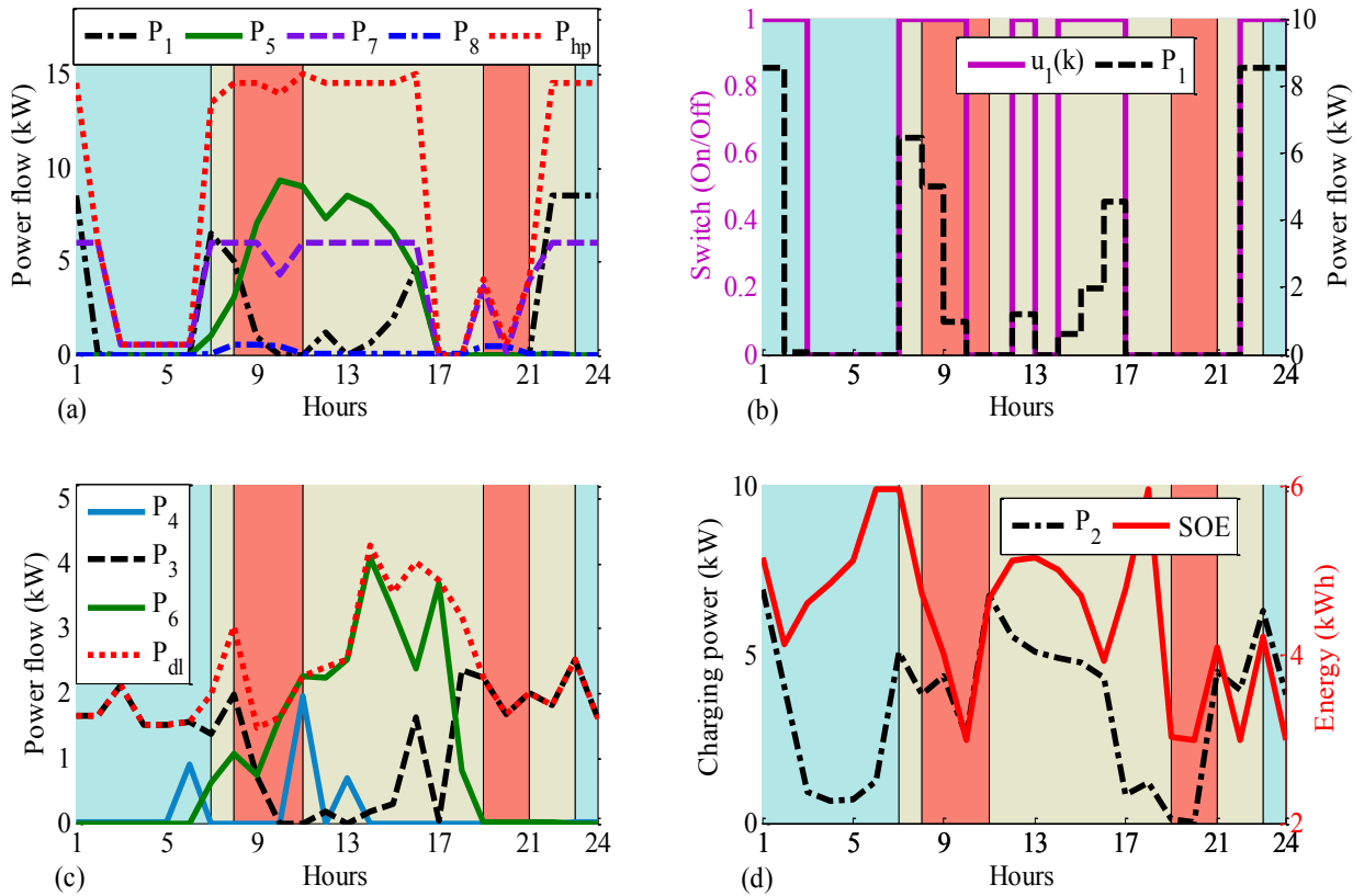
Figure 6: (a) OC of power to the HPWH; (b) OC switching to the HPWH; (c) Domestic load and solar sales ;(d) Battery SOE
