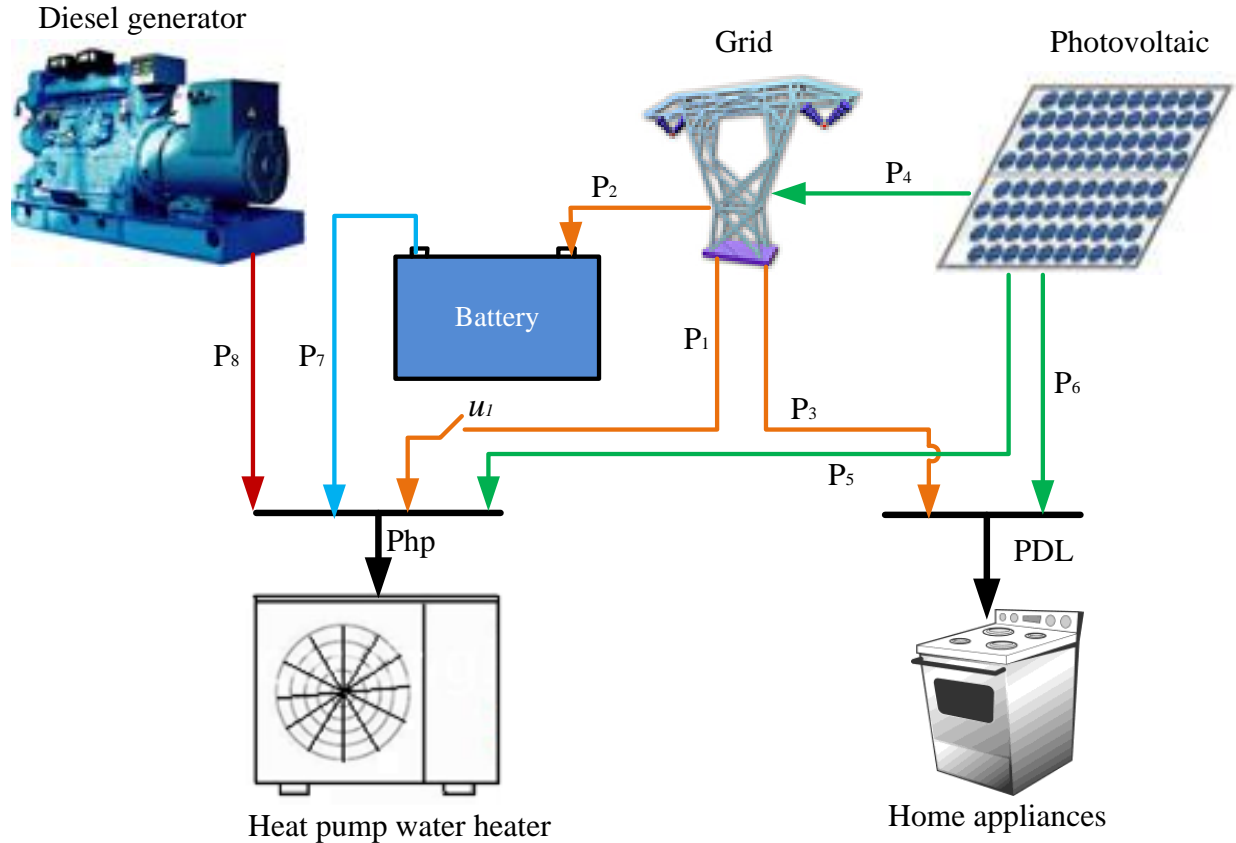
Figure 1: Schematic layout of the model.
