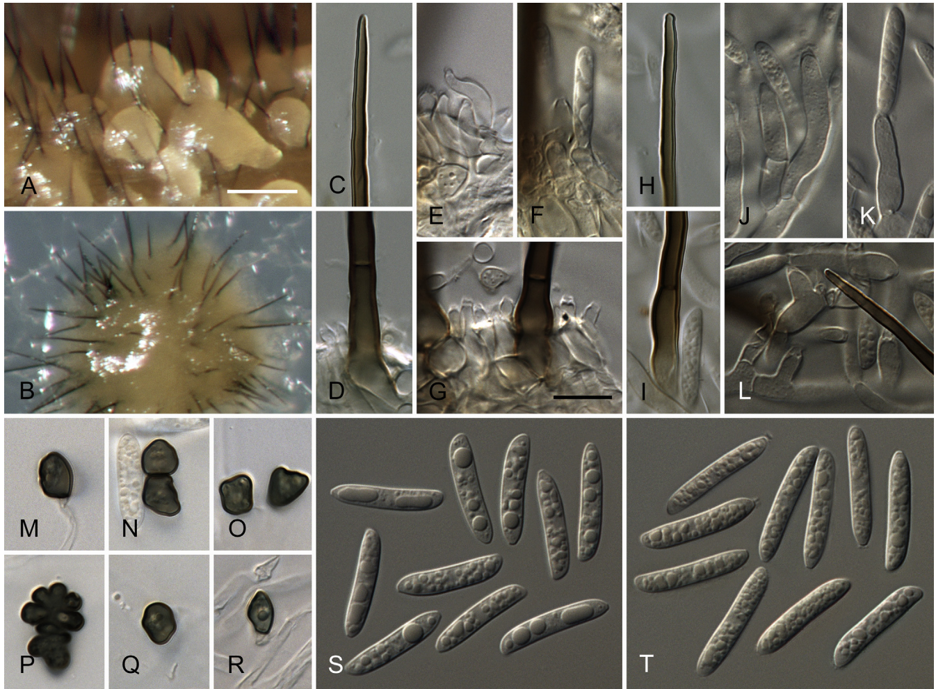
Fig. 7. Colletotrichum higginsianum (from ex-epitype strain IMI 349061). A–B. Conidiomata. C, H. Tip of a seta. D, I. Base of a seta. E–F, J–L. Conidiophores. G. Bases of seta and conidiophores. M–R. Appressoria. S–T. Conidia. A, C–G, S. from Anthriscus stem. B, H–R, T. from SNA. A–B. DM, C–T. DIC, Scale bars: A = 100 \mu m, G = 10 \mu m. Scale bar of A applies to A–B. Scale bar of G applies to C–T.
