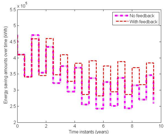
Figure 1: Energy performances of the maintenance plans with and without feedback in Optimal Balance case with sufficient budget.
