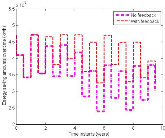
Figure 2: Energy performances of the maintenance plans with and without feedback in Energy Prior case with sufficient budget.
