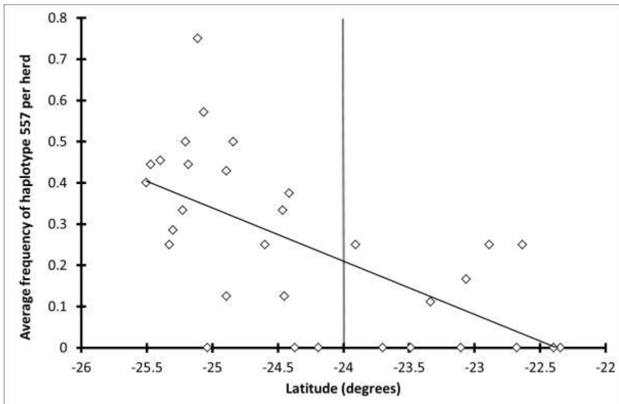
Figure S4: Cline of Y-chromosomal haplotype 557
