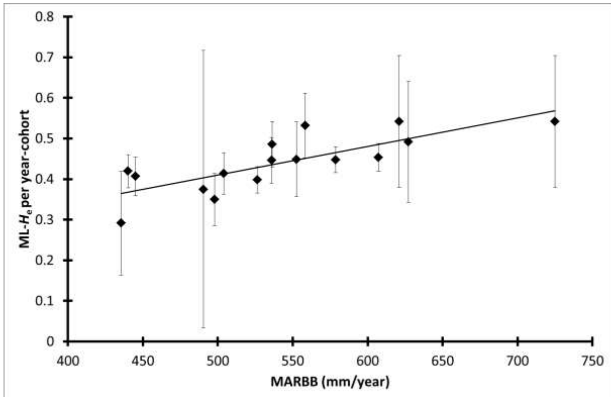
Figure S5: Regression between ML- H_e per year-cohort and preconception rainfall
