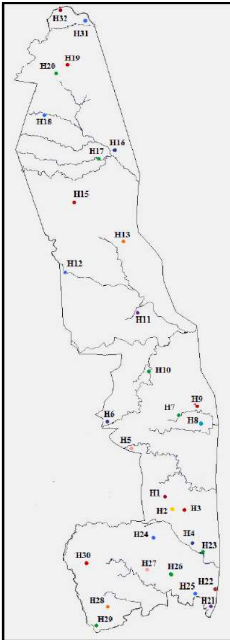
Figure S1: Map of Kruger National Park with localities of the sampled herds
