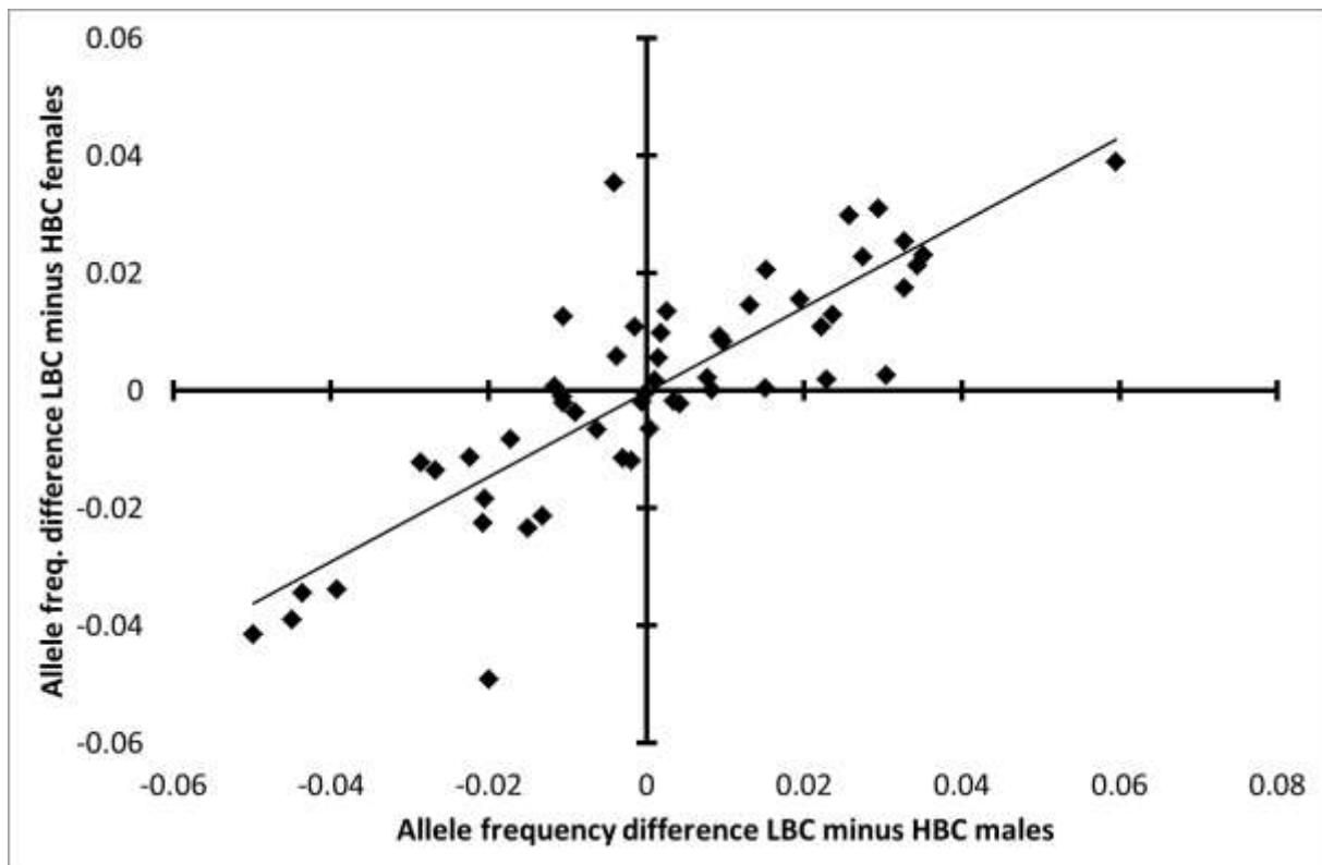
Figure S3: Positive correlation between males and females in LBC-minus-HBC allele frequency difference in the null model (Spearman rank correlation: \rho = 0.83 )
