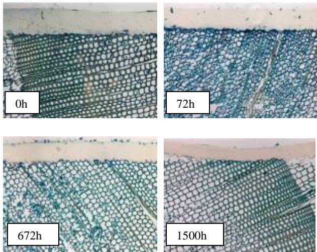
Figure 3 The light micrographs of transverse section of the heat-treated jack pine-coating containing bark extract and lignin stabilizer interface for different aging times
