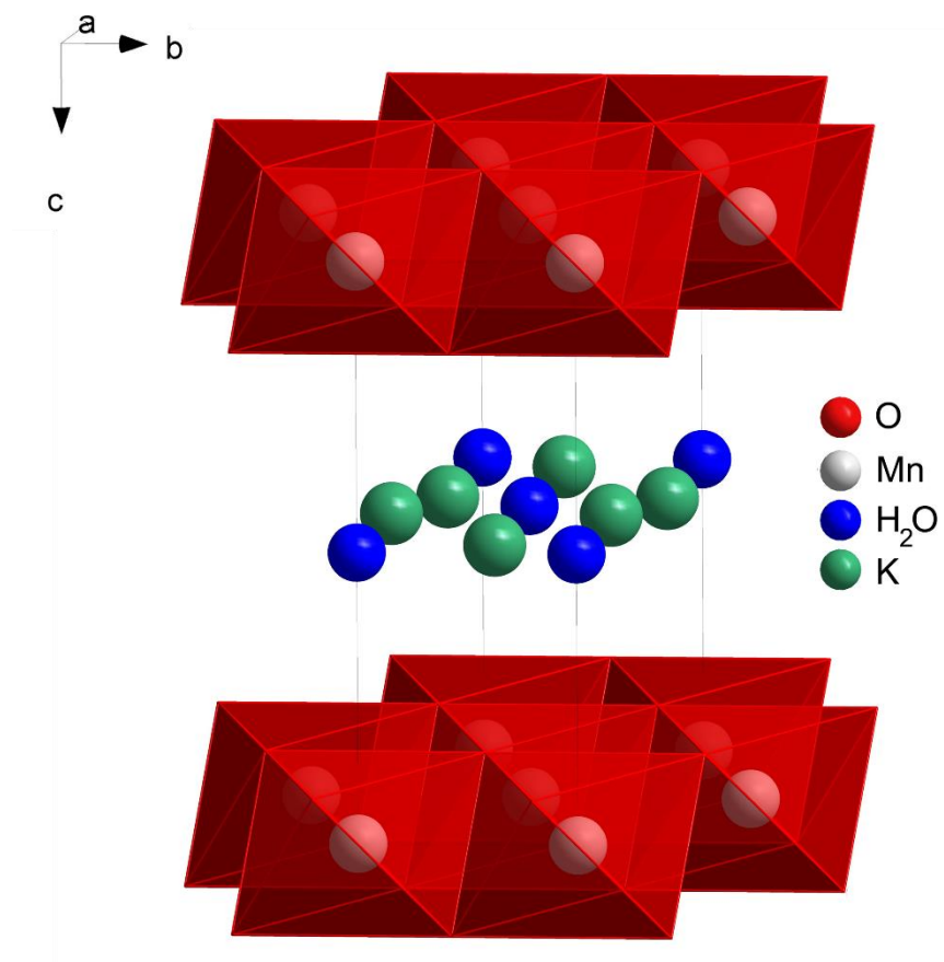
Fig. S1: Crystal structure of K_xMn_2O_4 \cdot yH_2O (birnessite).
