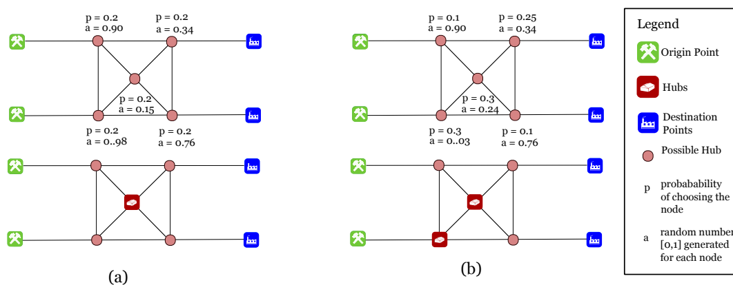
Figure 2.7: Multistart Heuristics
