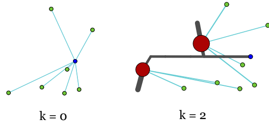
Figure 4.3: Multi-allocation of d_3 for k = 2
