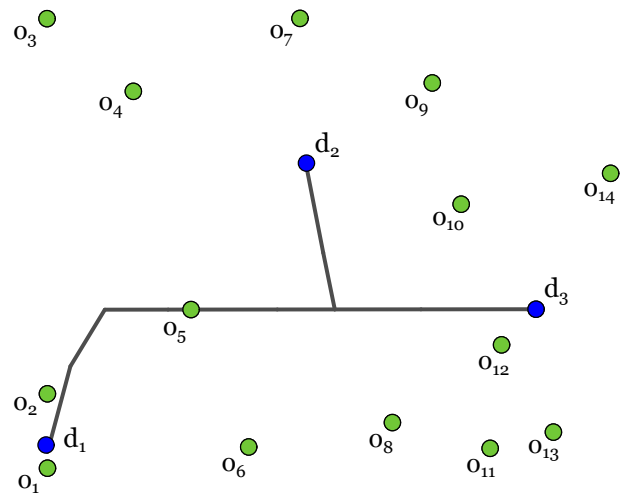
Figure 4.1: Test Case Study Area
