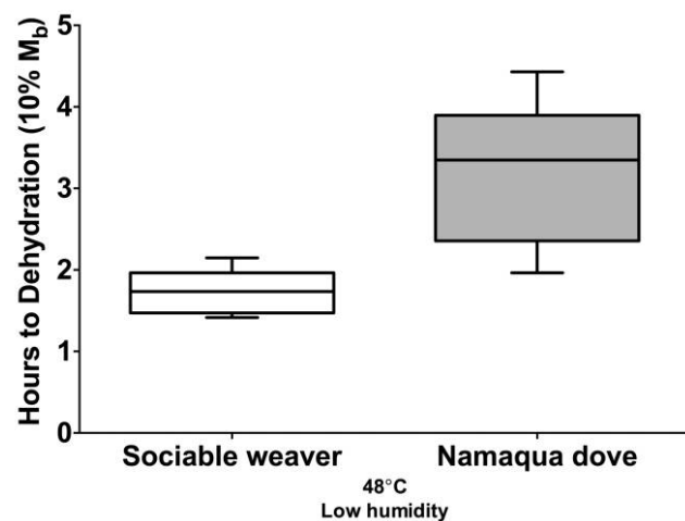
Figure 4. Time to mild dehydration, defined as 10% loss of mass as water, during heat exposure at 48°C and low humidity for sociable weavers and Namaqua doves.
