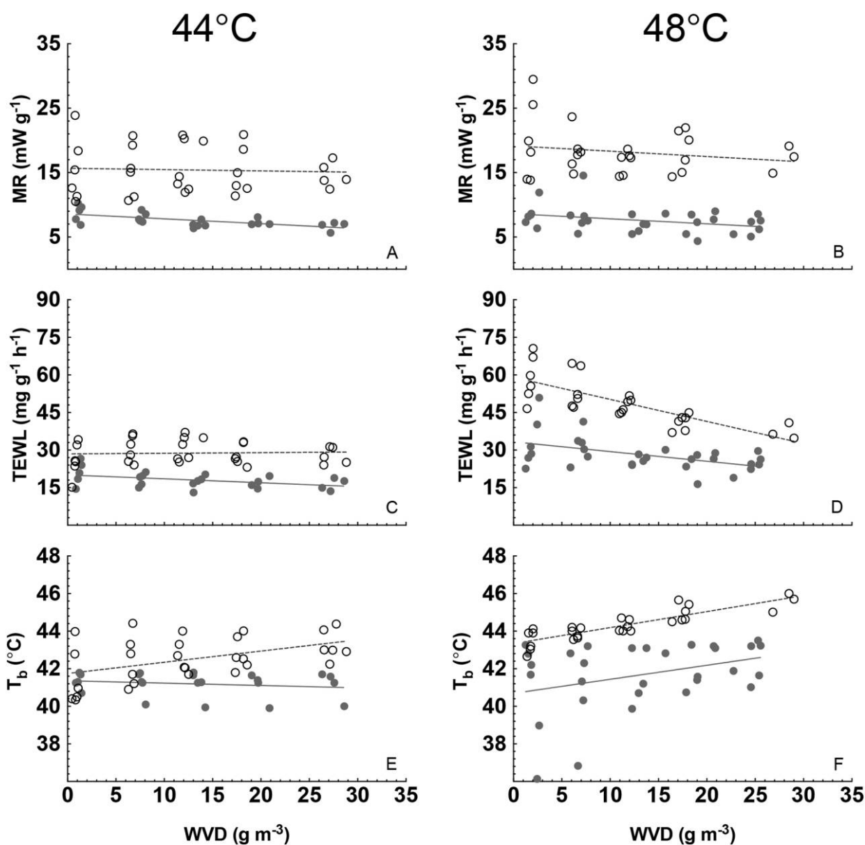
Figure 3. Comparison of the response of metabolic rate (A, B), evaporative water loss (C, D), and body temperature (E, F) to increasing humidity at common temperatures between sociable weavers (dashed lines) and Namaqua doves (solid lines). The left column corresponds to 44°C and the right column to 48°C, the two common exposure temperatures for the species studied. See text for statistical details and table 1 for parameter estimates.
