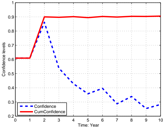
Figure 2: Annual and cumulative confidence levels.
