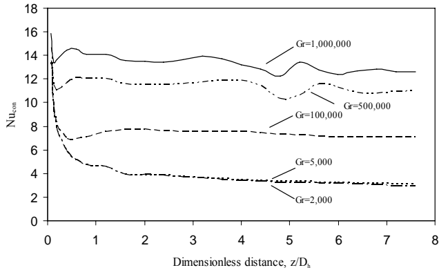
Figure 6 Variation of transverse average convective Nusselt number for AR=1 and \varepsilon = 0.85
