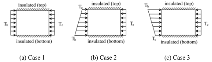
Figure 2 Duct wall heating configurations
