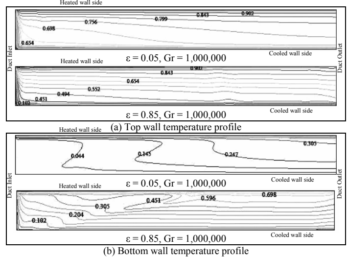
Figure 5 Dimensionless temperature contours at the top and bottom duct walls along duct length
