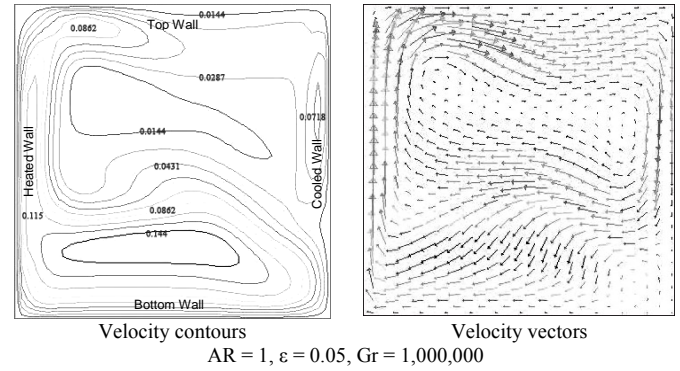
Figure 4 Axial velocity contours and vectors in duct
