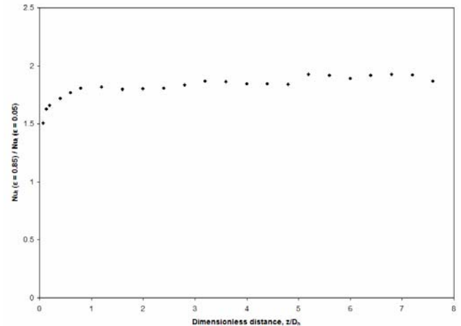
Figure 7 Variation of the total Nusselt number ratio with high ( \varepsilon = 0.85 ) and low ( \varepsilon = 0.05 ) emissivity for Gr = 1,000,000 .
