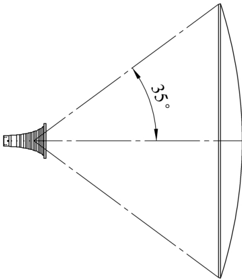
Fig. 11. The reflector antenna configuration.
