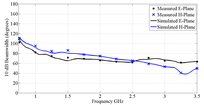
Fig. 8. Comparison between measured and simulated 10 dB beamwidth.
