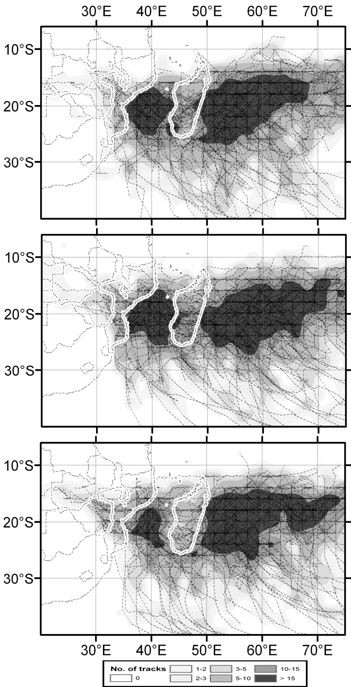
Fig. 5b Frequency of occurrence of TCLVs (shaded) per grid point for the period 1961-1990 as simulated by CCAM-MIROC (top), CCAM-GFDLcm2.0 (middle) and CCAM-GFDLcm2.1 (bottom). The actual tracks simulated by each CCAM ensemble member are also indicated
