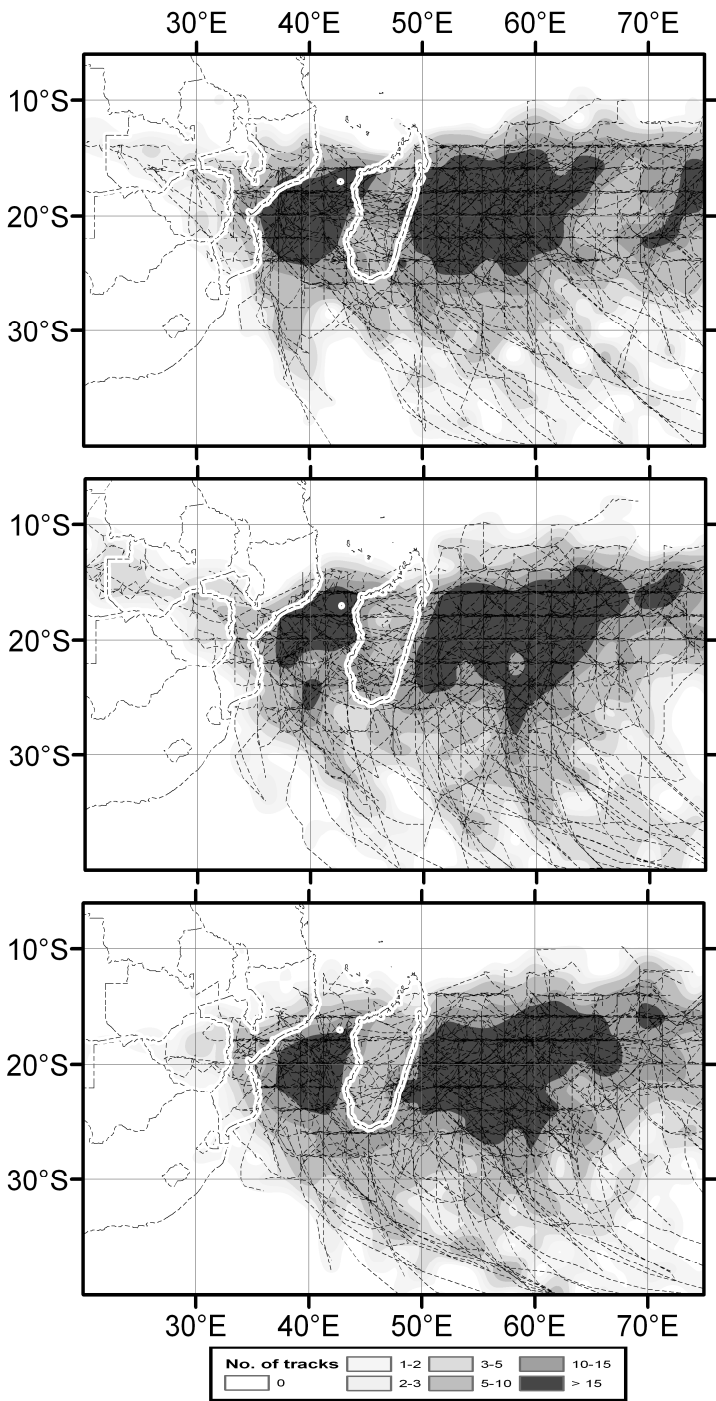
Fig. 5a Frequency of occurrence of TCLVs (shaded) per grid point for the period 1961-1990 as simulated by CCAM-CSIROMk3.5 (top), CCAMECHAM5 (middle), CCAM-UKHADcm3 (bottom). The actual tracks simulated by each CCAM ensemble member are also indicated
