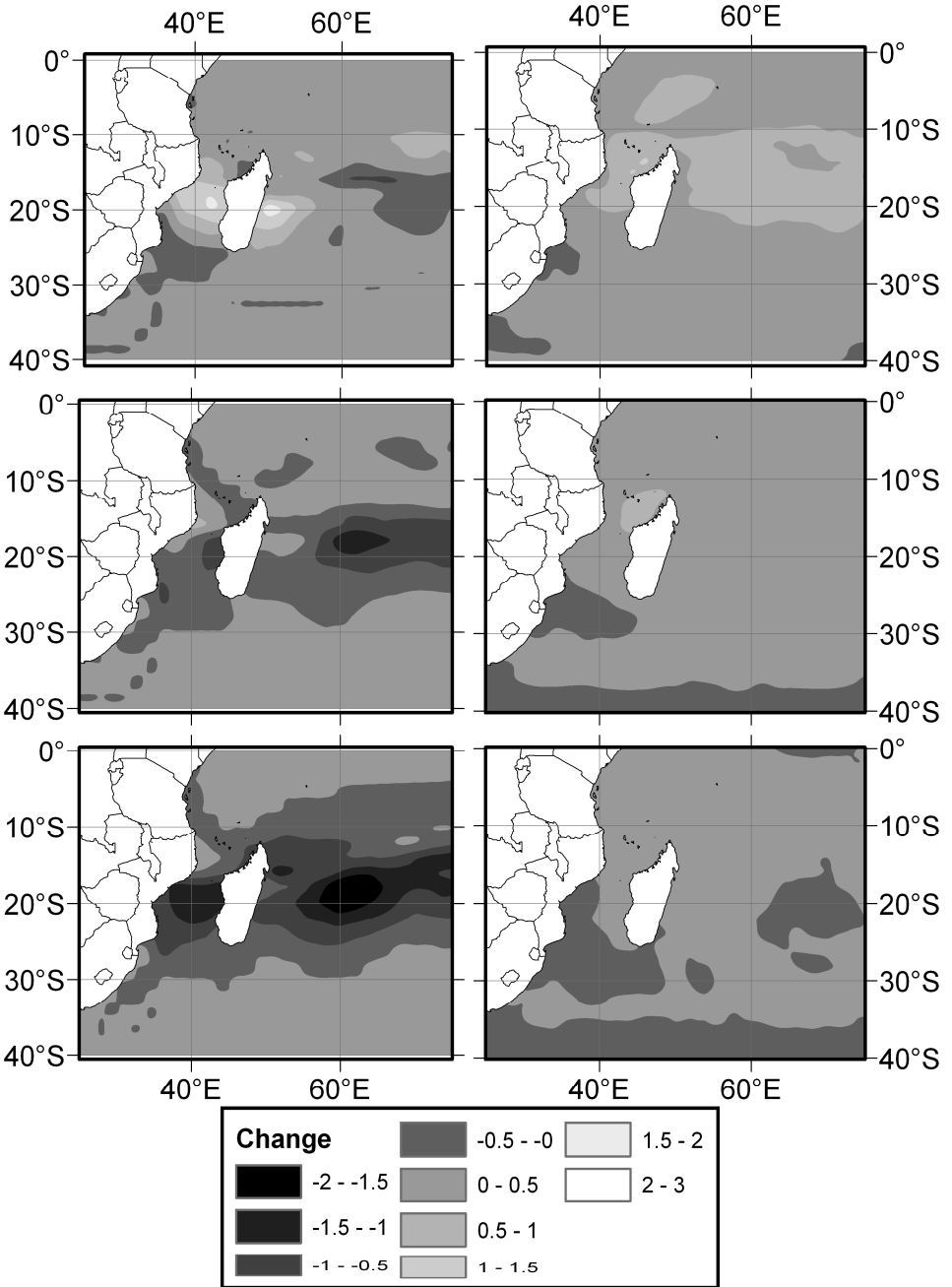
Fig. 15 75 th (top), 50 th (middle) and 25 th (bottom) percentiles of the change in the dynamic (left) and convective (right) components of the Convective Tropical Cyclone Genesis Index as calculated from the ensemble of CCAM members for the period 2071-2100 relative to 1961-1990
