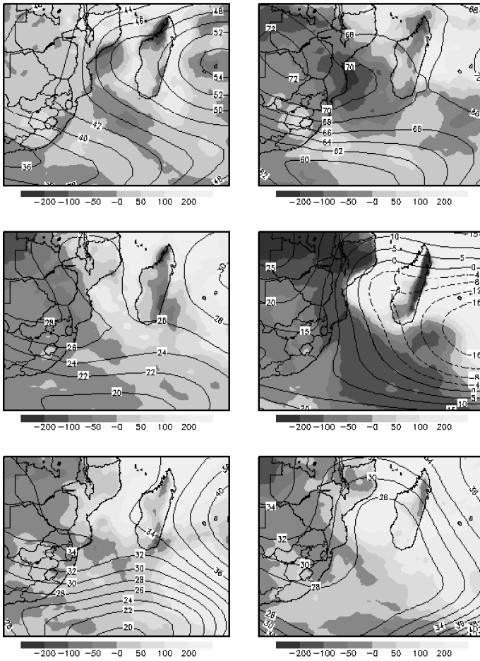
Fig. 12 Change in average January-March rainfall (shaded) and change in average heights at 700 hPa (contours) for 2071-2100 relative to 1961-1990 for CCAM-CSIROmk3.5 (top left), CCAM-ECHAM5 (top right), CCAM-UKHADcm3 (middle left), CCAM-MIROC (middle right), CCAM-GFDLcm2.0 (bottom left) and CCAM-GFDLcm2.1 (bottom right)
