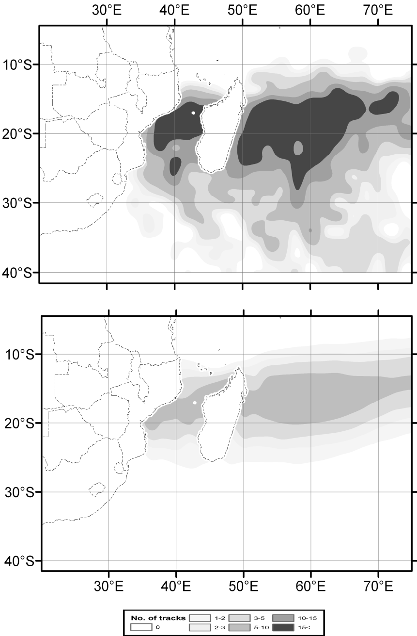
Fig. 13 Number of occurrences per grid point of TCLVs (top) assimilated by CCAM-MPI (Unit: total number of tropical cyclones passing per 2° grid point over a 30-year period) and CTCGP (Unit: approximate average twenty-yearly total number of tropical cyclones formed per 5° grid point) calculated for CCAM-MPI for the 1961-1990 period
