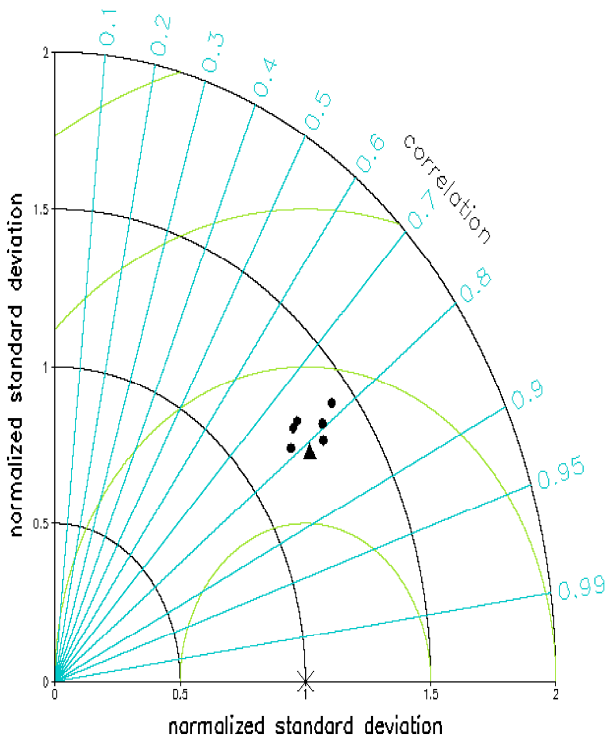
Fig. 6 Taylor diagram showing the statistical comparison of the simulation of TCLVs frequency of occurrence per grid point of the individual CCAM ensemble members (circles) and the CCAM ensemble mean (triangle) over the SWIO with the reanalysis distribution (cross)
