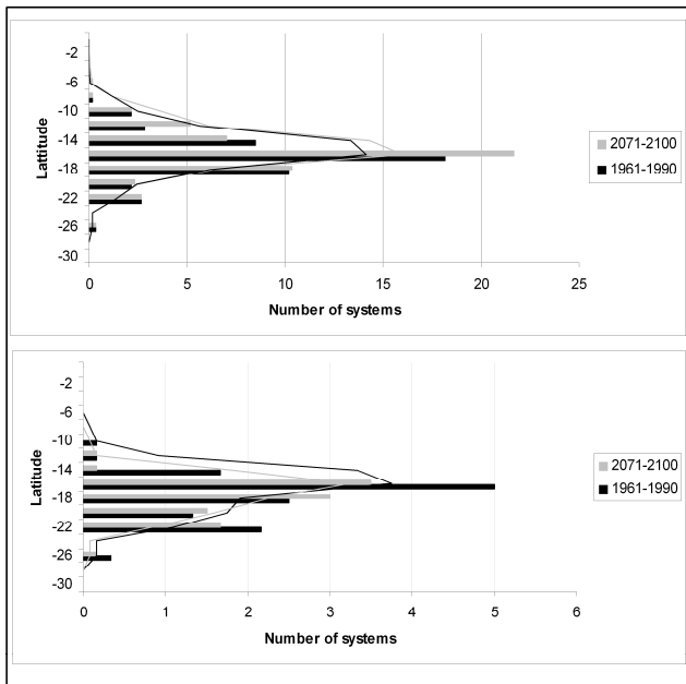
Fig. 10 Average number of warm core lows (top) and TCLVs (bottom) per 2° latitude interval making landfall over southern Africa from the SWIO as simulated for the 1961-1990 (black) and 2071-2100 (grey) periods by the CCAM ensemble. Lines representing the moving averages are also indicated
