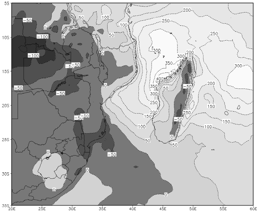
Fig. 11 CCAM ensemble average projected change in January-March rainfall between the 1961-1990 and the 2071-2100 periods
