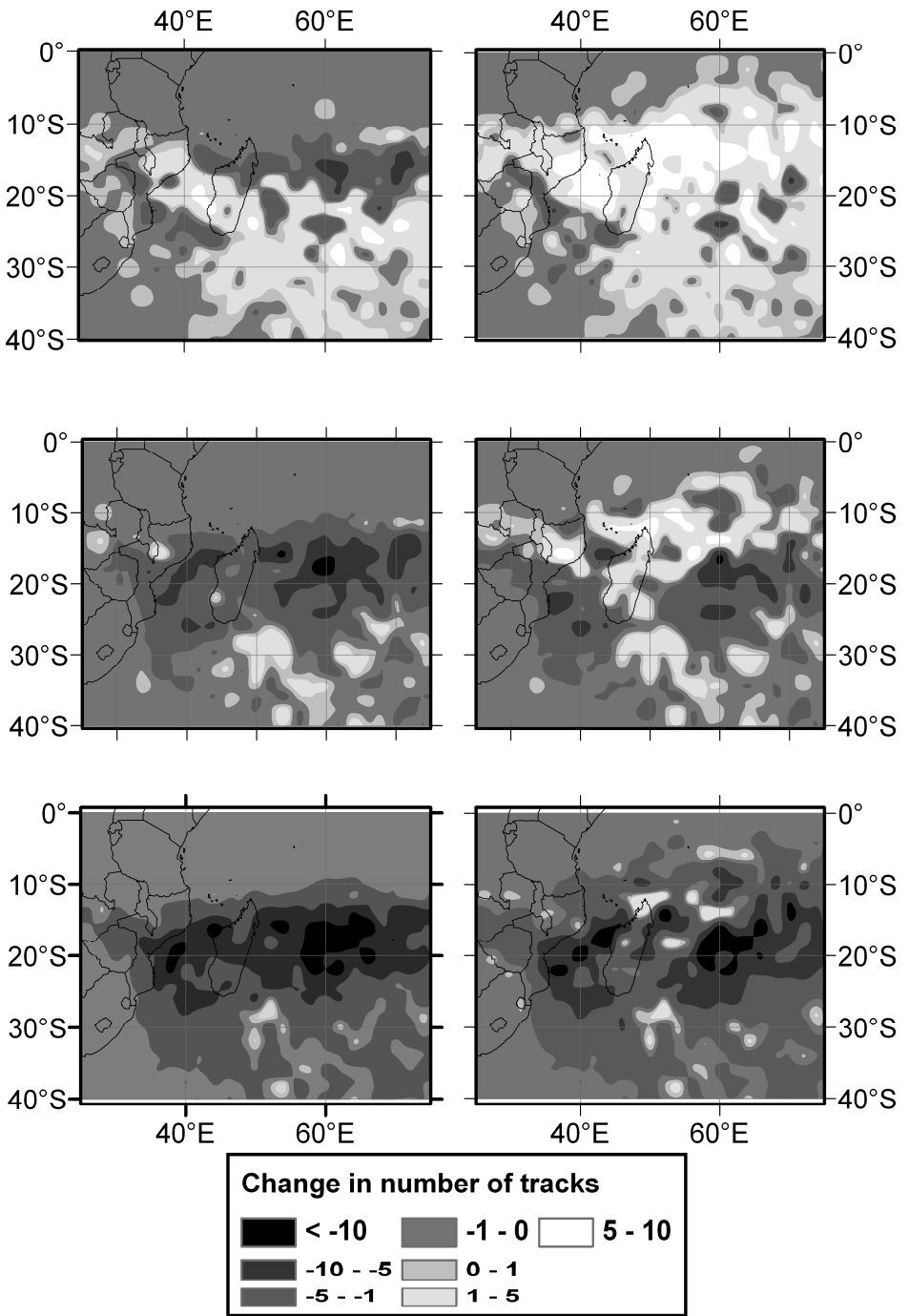
Fig. 9 75 th (top), 50 th (middle) and 25 th (bottom) percentiles of projected change in number of average January to March occurrences per grid point of TCLVs (left) and warm-core low pressure systems (right) as simulated by the CCAM ensemble for the 2071-2100 period relative to 1961-1990
