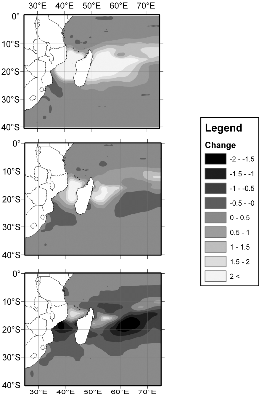
Fig. 14 75 th (top), 50 th (middle) and 25 th (bottom) percentiles of the change in the Convective Tropical Cyclone Genesis Parameter (Unit: approximate average twenty-yearly total number of tropical cyclones formed per 5° grid point) as calculated from the ensemble of CCAM members for the period 2071-2100 relative to 1961-1990
