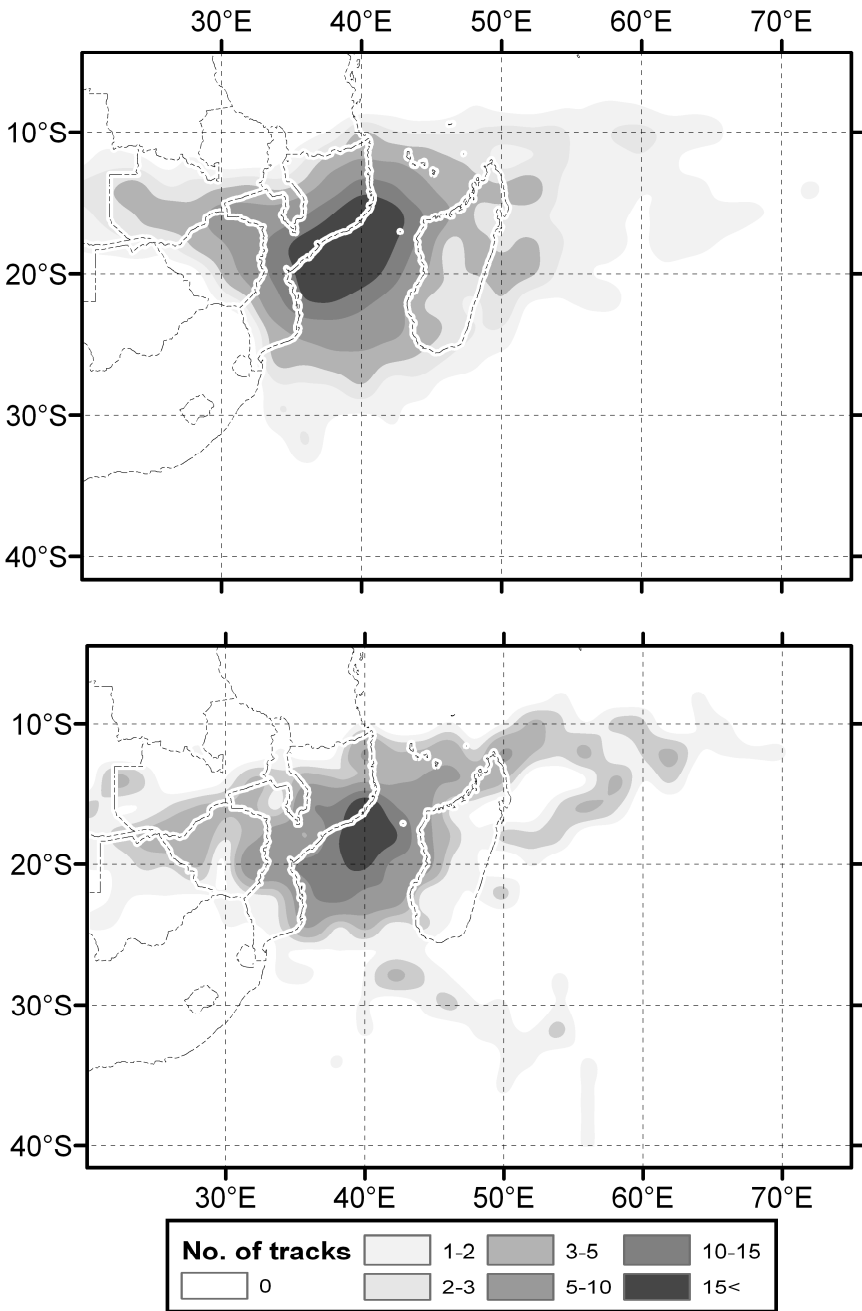
Fig. 7 Average frequency of occurrence of landfalling warm core closed lows per grid point (shaded), during January to March, as simulated by the CCAM ensemble average for 1961-1990 (top) and as according to NCEP Reanalysis data (bottom)
