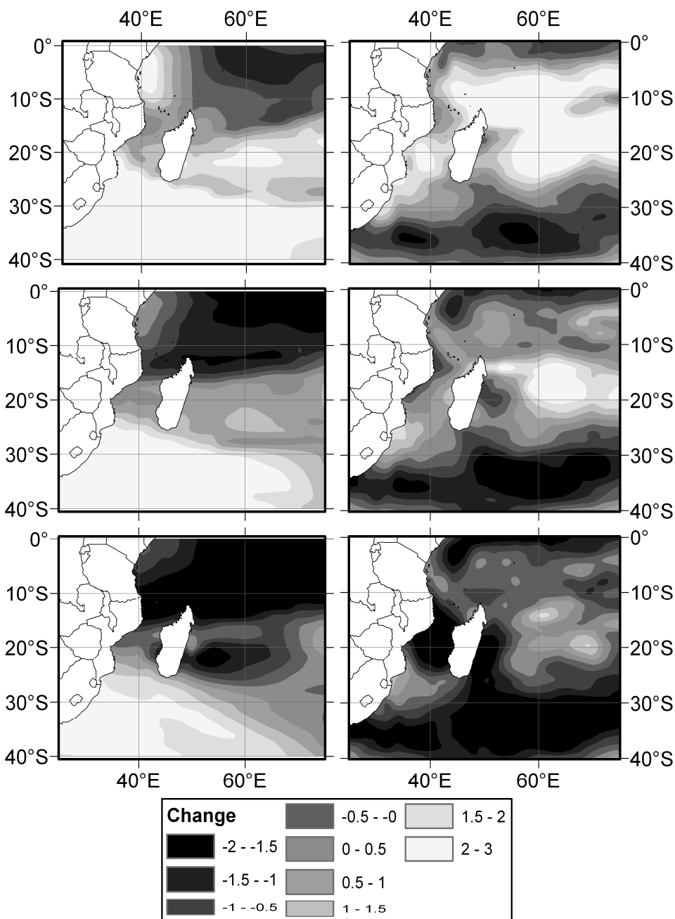
Fig. 16 75 th (top), 50 th (middle) and 25 th (bottom) percentiles of the change in the average wind shear ( \text{ms}^{-1} / 600\text{hPa} ) between 800 and 200hPa (left) and the change in vorticity ( 10^{-6}\text{s}^{-1} -right) as calculated from the ensemble of CCAM members for the period 2071-2100 relative to 1961-1990
