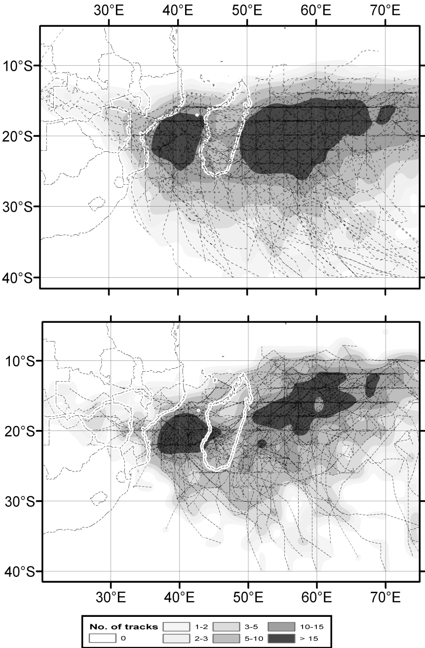
Fig. 3 Frequency of occurrence of TCLVs per grid point, as calculated from the ensemble average of the CCAM tracks (top, shaded) and as observed from the NCEP reanalysis data tracks (bottom shaded). The actual simulated tracks for the CCAMECHAM5 ensemble member is indicated (top), and similarly for the reanalysis data (bottom). Units are number of occurrences per grid point over the January to March period
