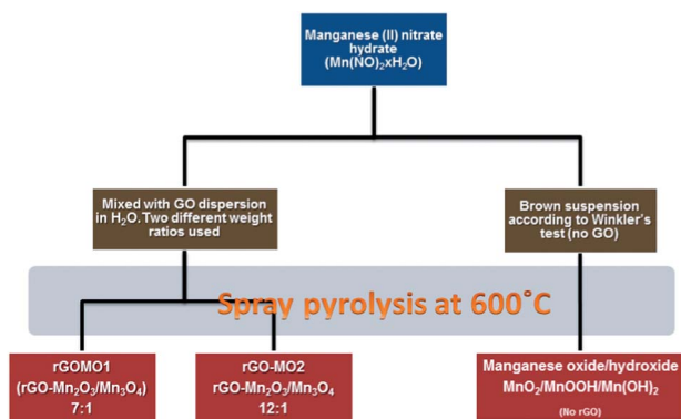
Fig. 1 Schematic diagram showing the experimental procedure for the formation of the Mn 2 O 3 –Mn 3 O 4 –rGO composites from manganese nitrate hydrate.
