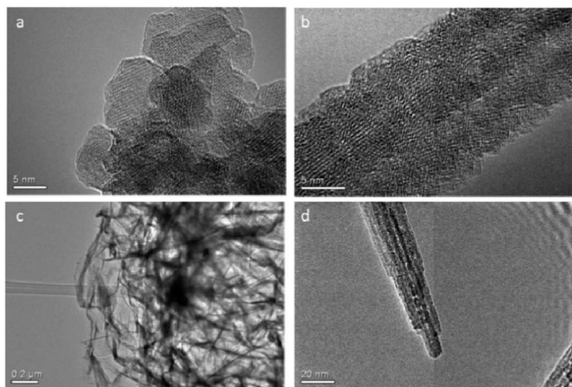
Fig. 4 HRTEM micrographs of manganese oxide–hydroxide showing (a) an agglomeration of nanoparticles which results in nanorods as shown in (b). The combination of rGO and Mn 2 O 3 –Mn 3 O 4 (c) and a high magnification, (d) rGOMO1.
