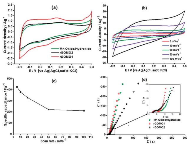
Fig. 6 (a) Cyclic voltammograms of the composites at 5 \text{ mV s}^{-1} . (b) Effect of scan rate on the shape of CV's of the best performing rGOMO1 electrode. (c) Variation of specific capacitance of the rGOMO1 composite electrode with scan rate. (d) Nyquist plots of the different composites showing the difference in charge transfer resistance in the high frequency region (inset). All experiments performed in 1 \text{ M NaOH} .
