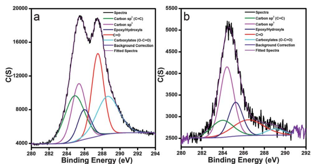
Fig. 5 Fitted XPS C1s spectra of (a) as-prepared GO sample and (b) spray pyrolyzed sample at 600 °C.
