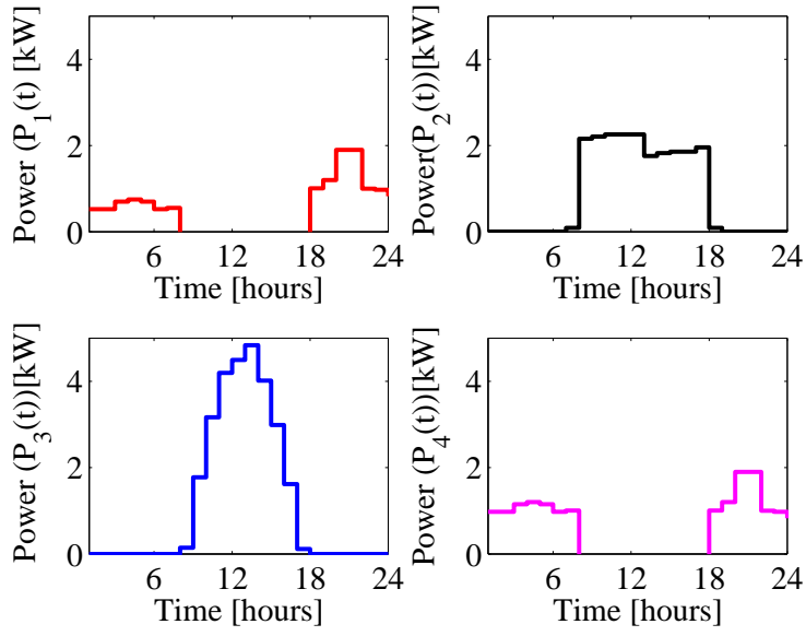
Figure 4: December weekend power flow
