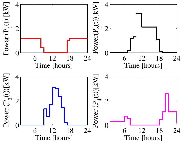
Figure 2: June weekend power flow
