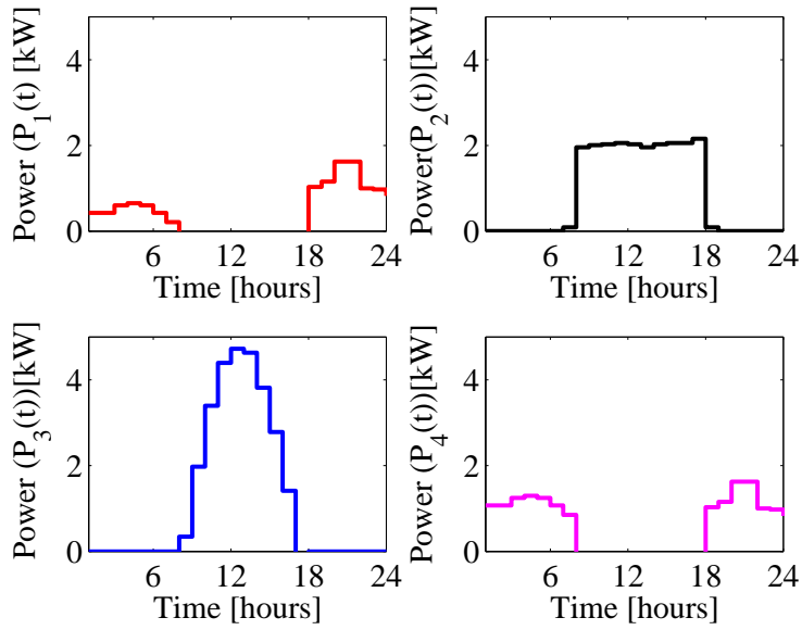
Figure 5: December weekday power flow
