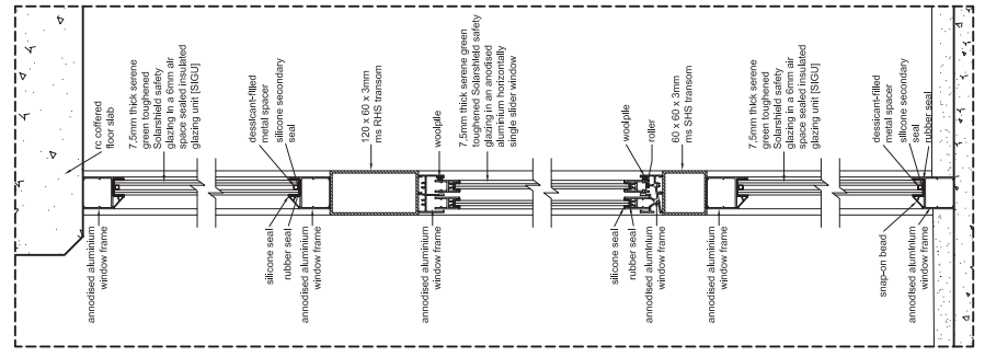
EXPLODED VIEW ALUMINIUM SINGLE SLIDER WINDOW PLAN DETAIL 1:4
