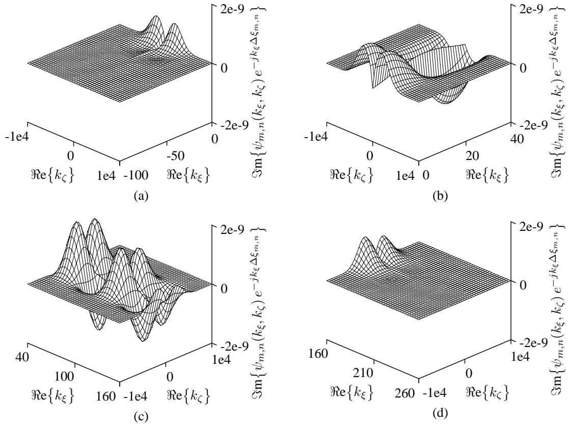
Figure 3.16 Integrand of Z_{m,n} , as a function of \Re\{k_{\xi}\} and \Re\{k_{\zeta}\} (but evaluated over the deformed k_{\zeta} integration contour), for rooftop basis and testing functions with: \Delta l_{ns} = \Delta w_{ns} = \Delta l_{ms} = \Delta w_{ms} = 1 mm, \phi_n = \phi_m = 0 , \vartheta = 45^\circ , \Delta\xi_{m,n} = 113.14 mm, h_{(1)} = 1.6 mm, h_{(2)} = 15 mm, \varepsilon_{r(0)} = \varepsilon_{r(2)} = 1 , \varepsilon_{r(1)} = 4 , \tan \delta_{\varepsilon(0)} = \tan \delta_{\varepsilon(1)} = \tan \delta_{\varepsilon(2)} = 0 and f = 1.91 GHz. (a) \Gamma_{\xi,1} part of k_{\xi} integration contour. (b) \Gamma_{\xi,2} part of k_{\xi} integration contour. (c) \Gamma_{\xi,3} part of k_{\xi} integration contour. (d) \Gamma_{\xi,4} part of k_{\xi} integration contour.
