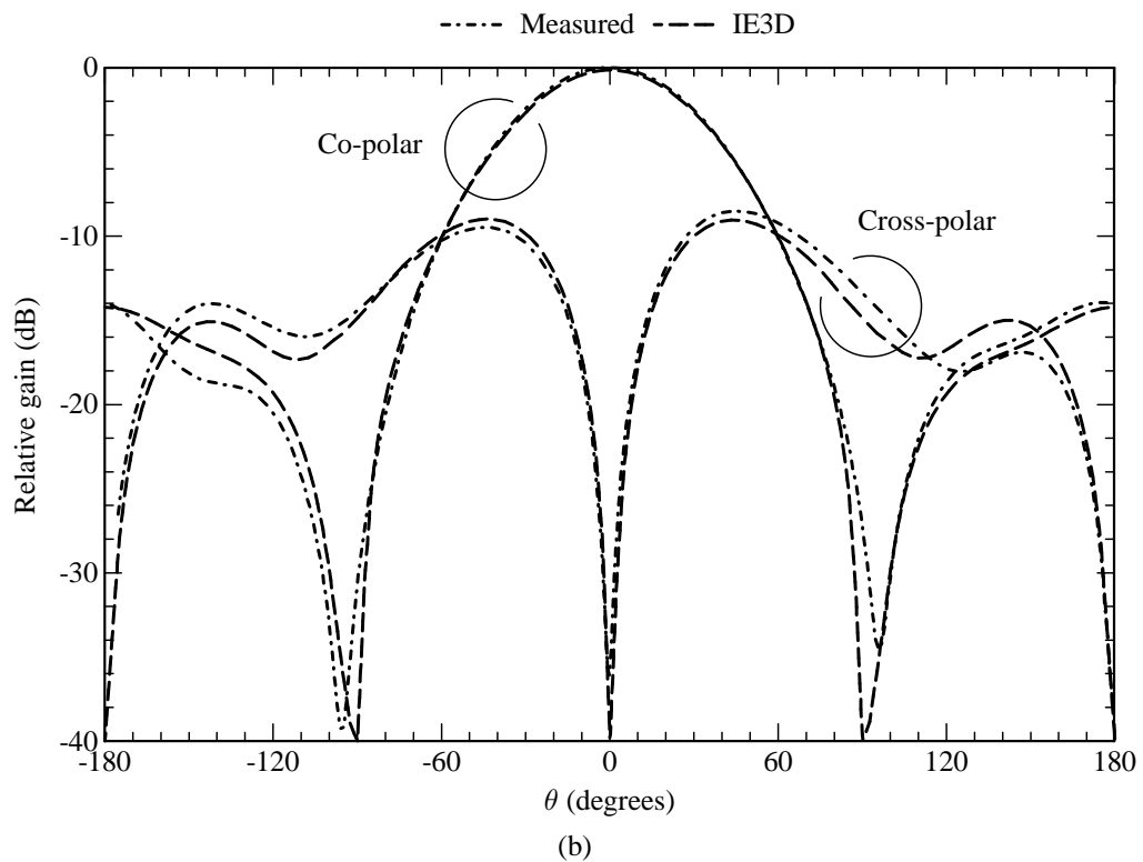
Figure 4.65 Radiation patterns (at 1.8 GHz) of the antenna element with an annular-ring resonant patch. (a) Co-polar radiation pattern in the E -plane ( \phi = 0^\circ ). (b) Co-polar and cross-polar radiation patterns in the H -plane ( \phi = 90^\circ ).
