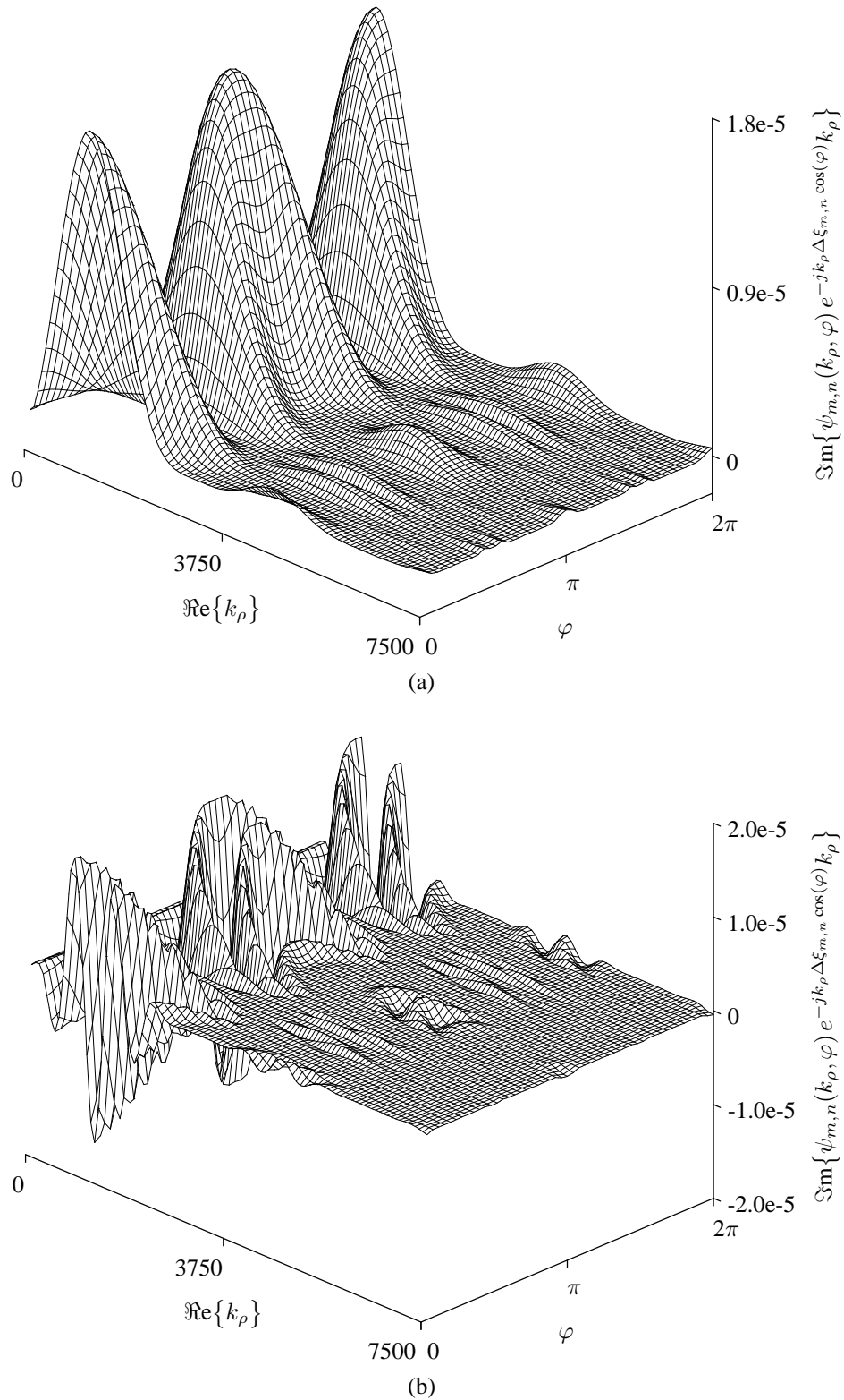
Figure 3.14 Integrand of Z_{m,n} , as a function of \text{Re}\{k_\rho\} (but evaluated over the deformed k_\rho integration contour) and \varphi , for rooftop basis and testing functions with: \Delta l_{ns} = \Delta w_{ns} = \Delta l_{ms} = \Delta w_{ms} = 2 mm, \phi_n = \phi_m = \vartheta = 0 , h_{(1)} = 1.6 mm, h_{(2)} = 15 mm, \epsilon_{r(0)} = \epsilon_{r(2)} = 1 , \epsilon_{r(1)} = 4.25 , \tan \delta_{\epsilon(0)} = \tan \delta_{\epsilon(2)} = 0 , \tan \delta_{\epsilon(1)} = 0.02 and f = 1.8 GHz. (a) Completely overlapping basis and testing functions ( \Delta \xi_{m,n} = 0 ). (b) Separated basis and testing functions with \Delta \xi_{m,n} = 8 mm.
