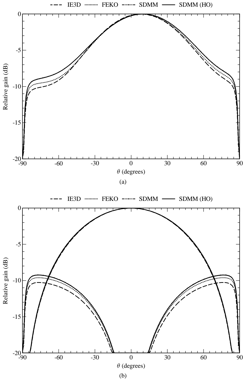
Figure 4.19 Radiation patterns (at 1.8 GHz) of the antenna element with a circular capacitor patch. Parameters: b = 4.5 mm and d = 4 mm. (a) Radiation pattern in the E -plane ( \phi = 0^\circ ). (b) Radiation pattern in the H -plane ( \phi = 90^\circ ).
