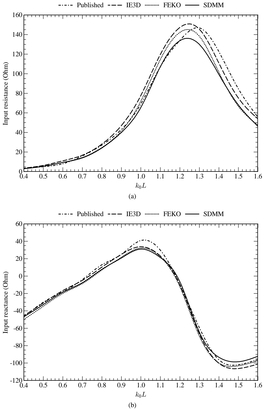
Figure 4.2 Input impedance of a probe that is embedded within a grounded substrate. Parameters: a = 1.5 mm, h = 0.3\lambda_0 , \epsilon_r = 3.9 and \tan \delta_\epsilon = 0 . (a) Input resistance. (b) Input reactance.
