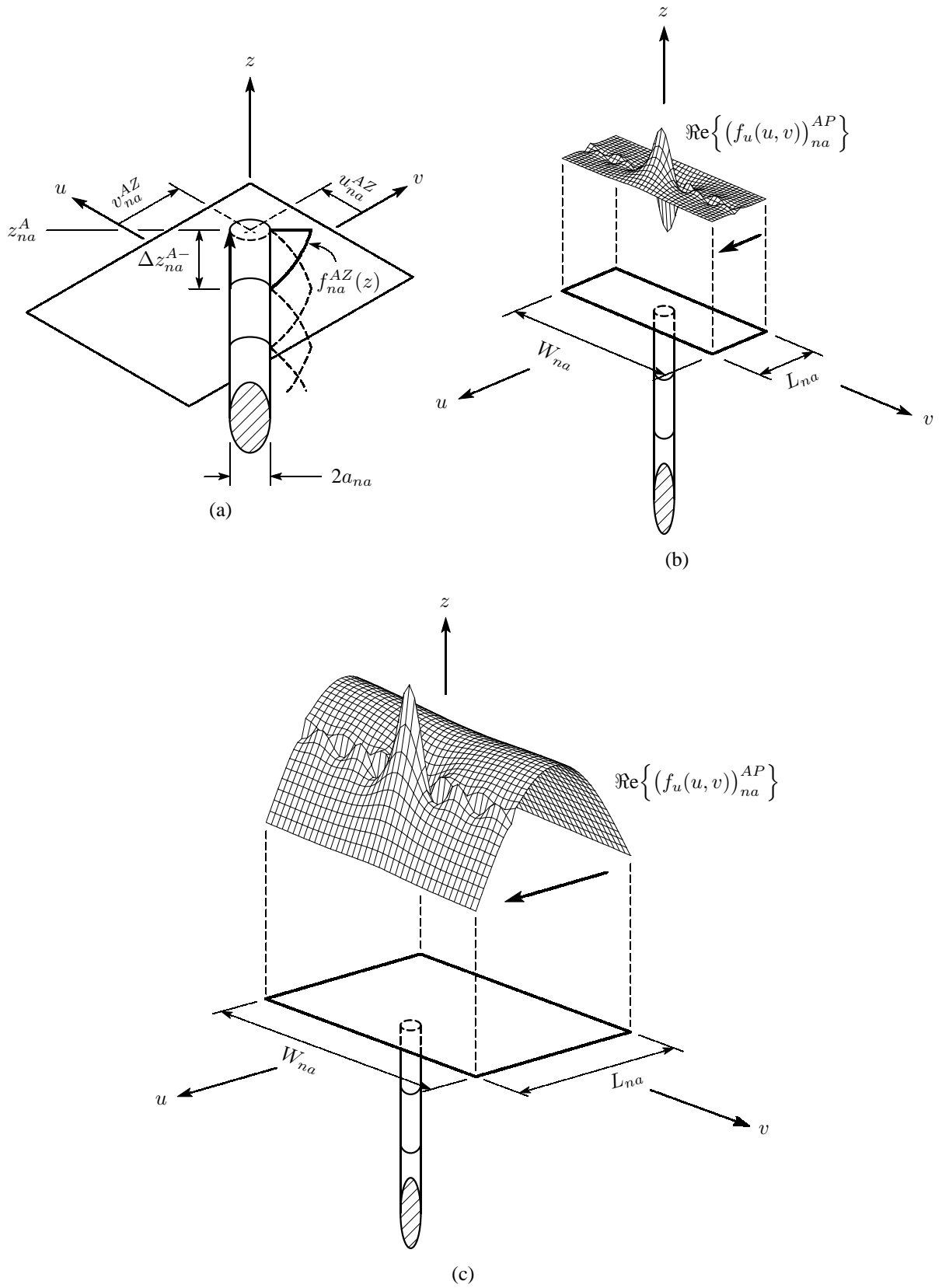
Figure 3.10 Rectangular attachment mode na . (a) Probe part of the attachment mode. (b) Patch part of the attachment mode for a small patch. (c) Patch part of the attachment mode for a resonant patch.
