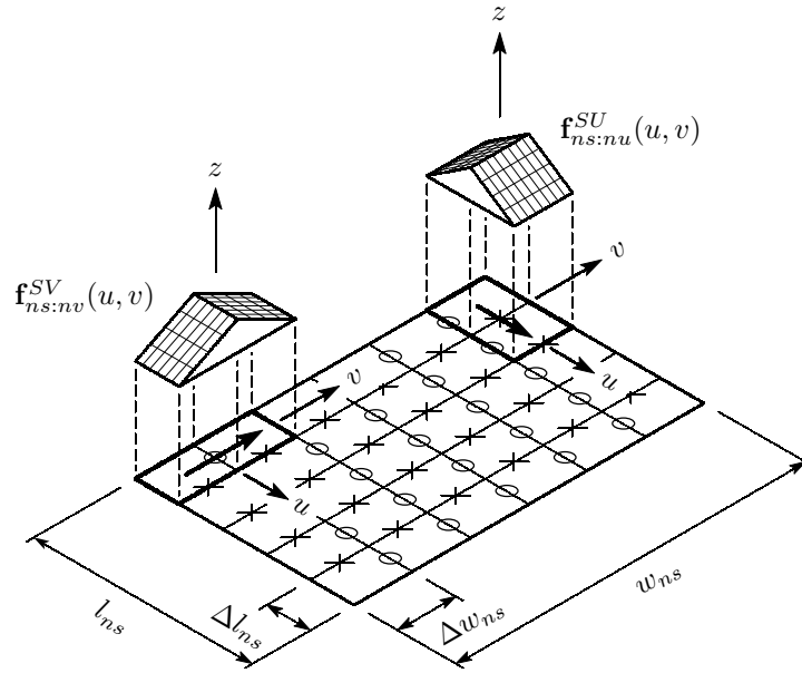
Figure 3.8 Subdomain rooftop basis functions on rectangular capacitor patch n_s .
