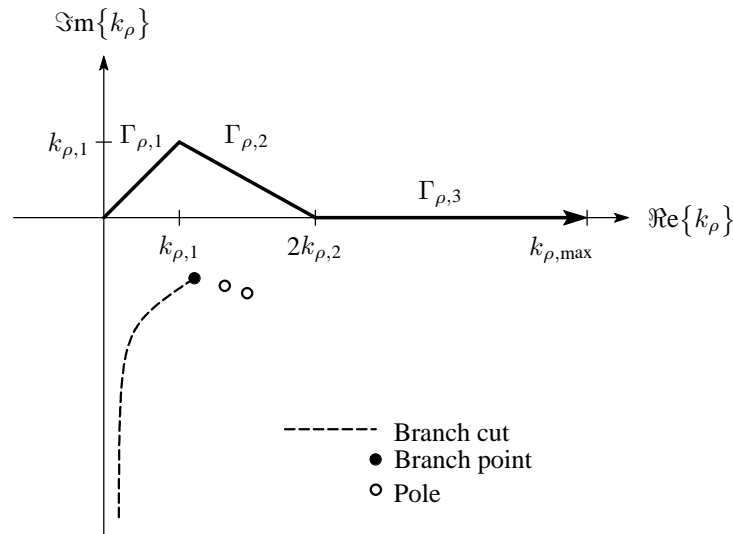
Figure 3.13 Integration path in the complex k_\rho plane for overlapping basis and testing functions.
