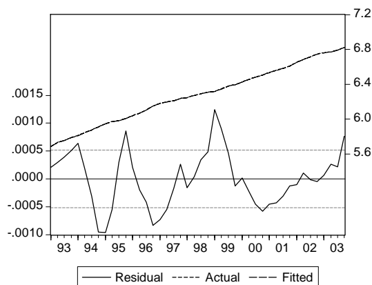
Figure 2.10: Residual Plot
