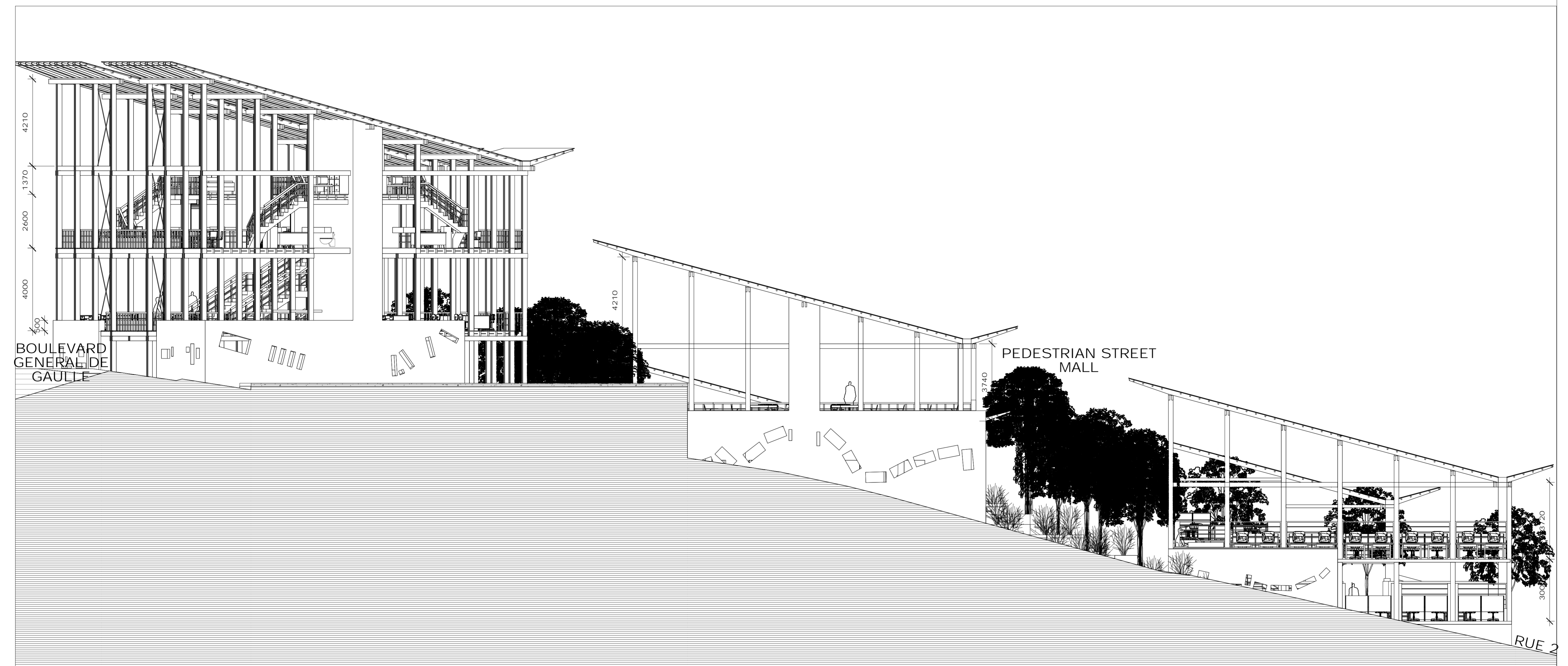
SOUTH ELEVATION - 1:100 - 2/20/A0
