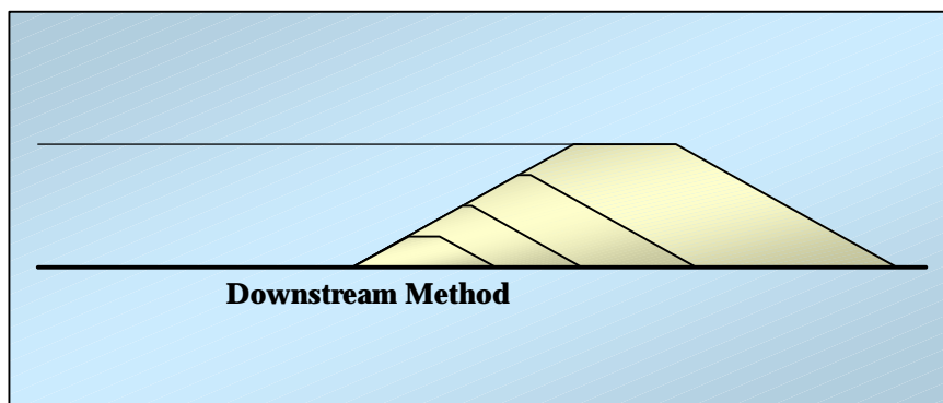
Figure 2.18: Downstream depositional method (Vick, 1987)
