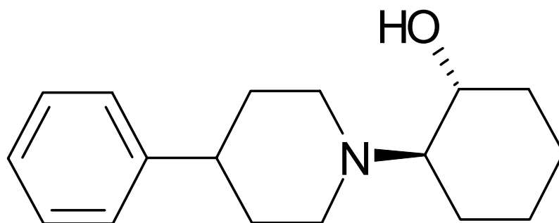
Figure 9.1 L-(-)-vesamicol
