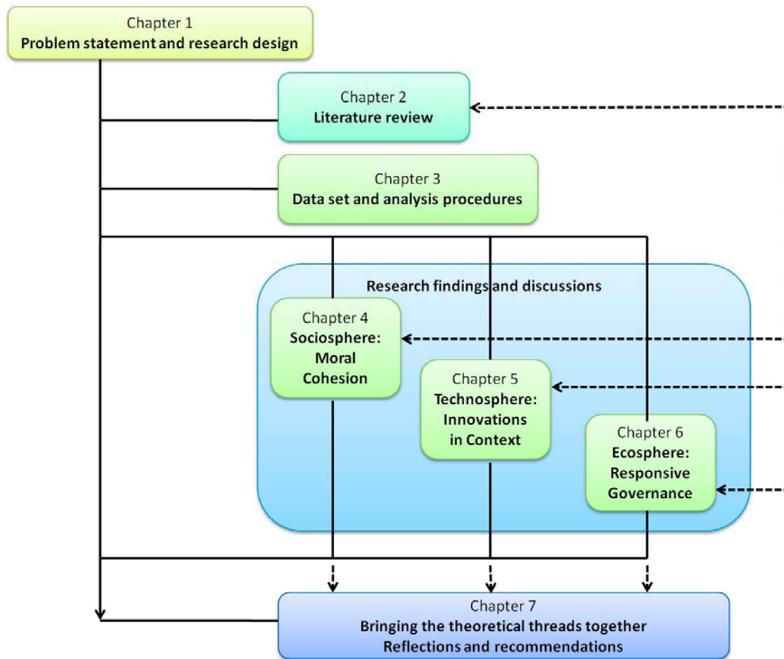
Figure 1-10: Thesis outline
