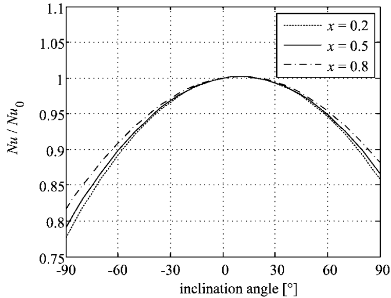
Fig. 10. Effect of the inclination angle on the heat transfer for R134a condensing in a microfin 8.92 mm inside diameter tube at mass fluxes from 54 to 107 kg/m 2 s (Akhavan-Behabadi et al., 2007).
