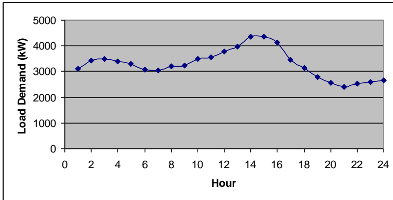
Fig. 12. Typical summer day load demand for the village (July 14, 2005).
