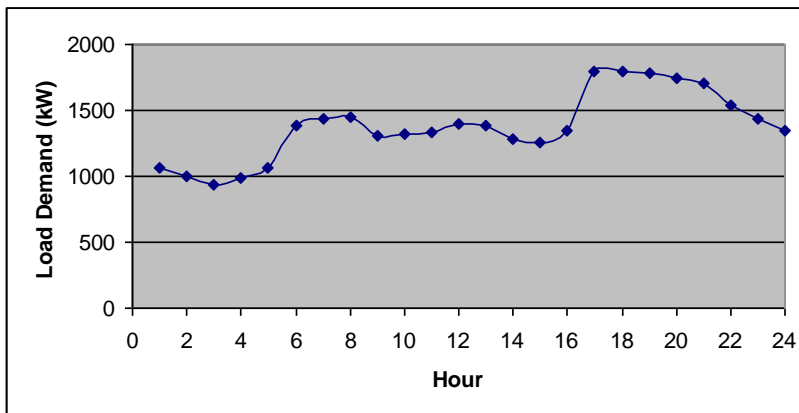
Fig. 13. Typical winter day load demand for the village (January 03, 2005).
